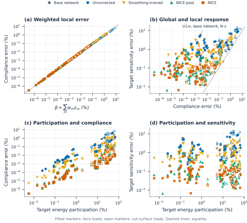
Figure 10: Participation-weighted compliance error and local sensitivity. Each point is one load for one predictor–configuration combination: 411 observations from 52 combinations of the base network, Uncorrected, Smoothing-trained, NICE-post and NICE in Table ST09, excluding L1. Filled markers denote face loads and open markers cut-surface loads. (a) Compliance error against \beta = \sum_m w_m \varepsilon_m , with w_m = q_m^T S_m q_m / C and \varepsilon_m = q_m^T (\hat{S}_m - S_m) q_m / (q_m^T S_m q_m) , evaluated at the exact assembled retained displacement; only the learned target contributes to \beta . (b) Compliance and target-cell sensitivity errors under the same loads; the annotation identifies the base network on U1/x under the neighbour-z load. Dashed lines denote equality. (c,d) The two response errors versus the target's exact energy participation.
