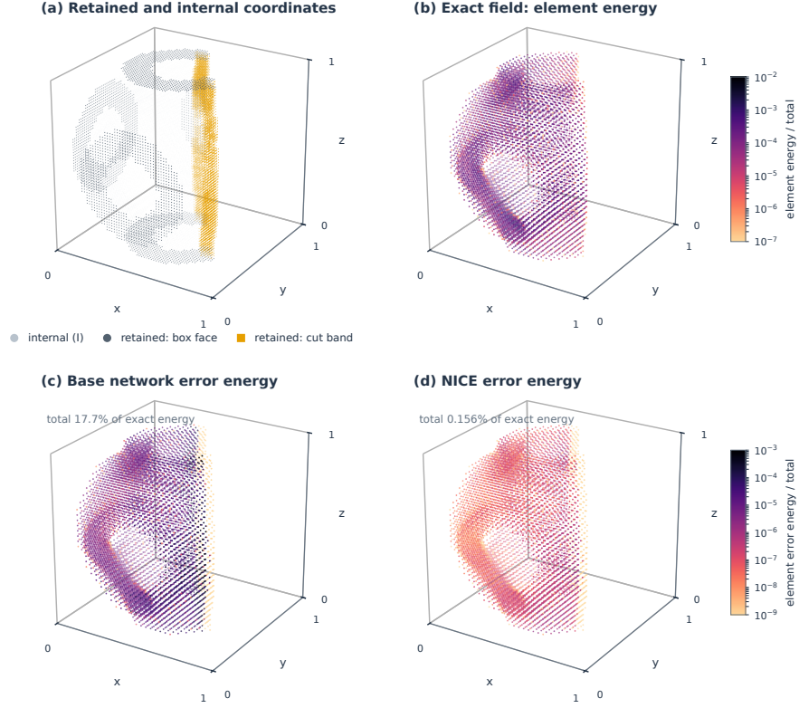
Figure 7: Retained coordinates and spatial distribution of the extension error in M1. (a) Retained box-face coordinates, retained cut-band coordinates and internal coordinates. (b) Bulk element energies of the exact field under one consistent-traction direction, relative to its total. (c,d) Bulk element energies of the error of the base network and of NICE for the same retained displacement, on a common colour scale. Cut-band elements carry no error because their coefficients are retained.
