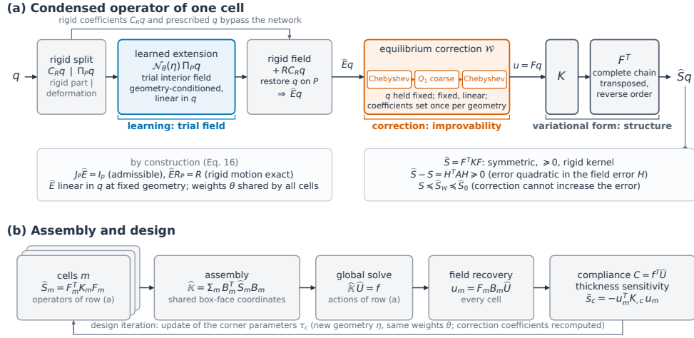
Figure 2: Learned displacement extension, equilibrium correction and variational assembly. (a) Rigid motion is separated from the retained displacement before the deformation is extended by the network. The rigid field is reconstructed and the prescribed retained values are restored; correction then reduces internal imbalance at fixed retained displacement. (b) Applying the local stiffness and the complete extension transpose gives the work-conjugate retained force. The assembled solution supplies the inputs for local field recovery. The neural extension is detailed in Figure 3 and Section 4.4; Sections 4.2 and 4.3 define the internal correction.
