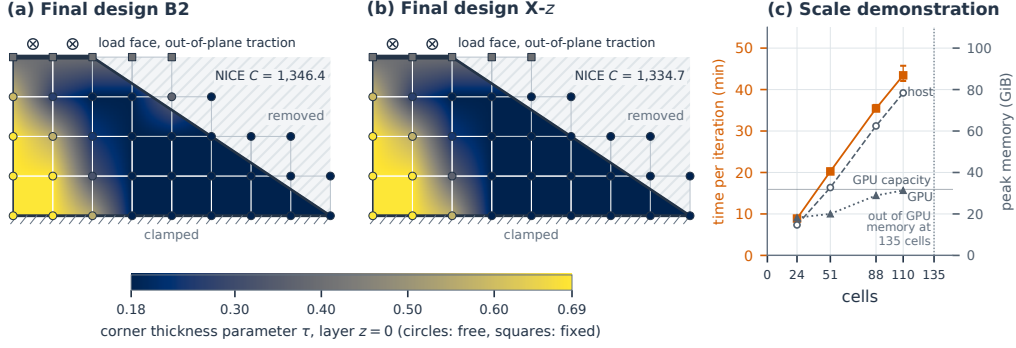
Figure 13: Final plate designs and scale demonstration. (a,b) Corner thickness parameters of the final designs B2 and X-z, drawn with the long side horizontal, layer z = 0 (layer z = 1 differs by at most 7.0 \times 10^{-4} in B2 and 2.0 \times 10^{-4} in X-z); circles: design variables; squares: vertices in the plane of the loaded face, held fixed; vertices drawn in the removed region are corners of cut cells. \otimes : load face, traction normal to the plate. (c) Scale demonstration on plates with the geometry and load of B1: time per design iteration (mean; bars: range over the timed iterations), peak host memory of the main process and peak GPU memory in use, against the number of cells; at 135 cells the factorisation of K_{PP} on the GPU ran out of device memory. Plate compliances are NICE values; exact checks of the plate designs in Table 6 and Table ST27.
