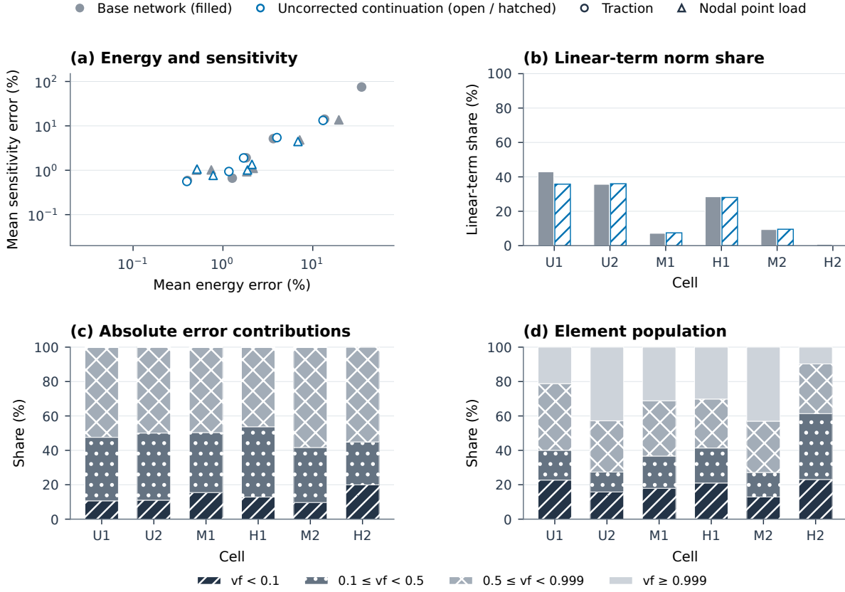
Figure S03: Sensitivity-error diagnostics. (a) Paired mean energy and sensitivity errors for responses to traction loads and nodal point loads, using six cells of the base network and five of the Uncorrected continuation. (b) Linear-term norm fraction \|D_1\|_F / (\|D_1\|_F + \|D_2\|_F) under traction loads, where D_1 + D_2 is the sensitivity-error matrix over all eight design components and evaluated test displacements. (c,d) Fractions of absolute elementwise sensitivity-error contributions and of element counts in four mutually exclusive material-volume-fraction groups for the base network under traction loads. Each error group sums absolute contributions over its elements, design components and test displacements before normalisation by the total. Filled markers identify the base network. In (a,b), open markers and hatched bars identify the Uncorrected continuation, which is shown for U1, U2, M1, H1 and M2 (Table ST05a).
