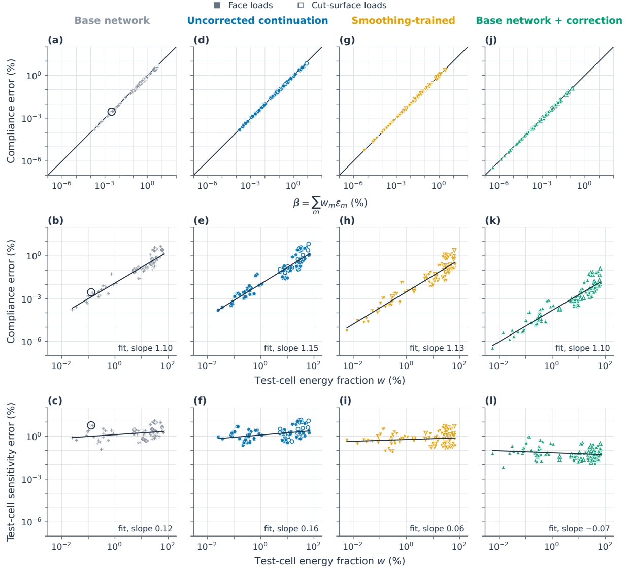
Figure S04: The other four variants follow the relations of Figure 11. The counterpart of Figure 11 for (a–c) the base network, (d–f) the Uncorrected continuation, (g–i) the Smoothing-trained variant and (j–l) Base network + correction, which applies the correction at deployment. One point per load in the configurations evaluated for each variant (54, 87, 96 and 114 loads; Tables ST08 and ST09); filled markers denote face loads and open markers cut-surface loads. Top row: compliance error against \beta ; lines denote equality. The ratio of compliance error to \beta lies between 0.80 and 0.98, 0.79 and 0.99, 0.92 and 0.99, and 0.96 and 1.006 for the four variants; the six ratios above 1 correspond to at most 1.3 \times 10^{-9} of the compliance. Middle and bottom rows: compliance error and test-cell sensitivity error against the exact energy fraction w of the test cell; lines are least-squares fits in logarithmic coordinates, with the slope given in each panel. All panels share the error axis. The circled load in (a–c) is U1/x under the z traction load on the face of the neighbouring cell; its values are given in the note to Table ST08.
