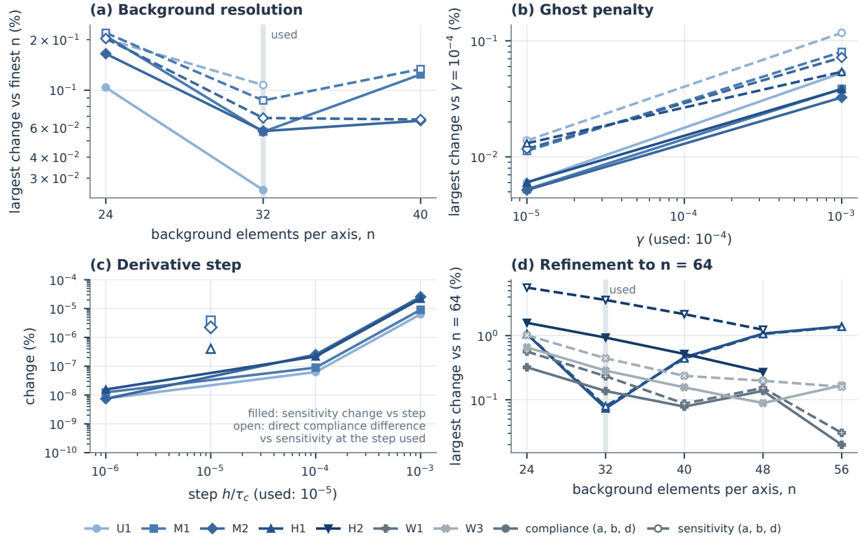
Figure S01: Verification of the CutFEM reference. Single cells clamped on one cell face and loaded by unit traction loads on another face in the three Cartesian directions. In (a), (b) and (d), solid lines with filled markers give the compliance and dashed lines with open markers the thickness sensitivity, each as the largest relative change over the three loads. (a) Change against the finest background resolution computed for U1 ( n = 40 ) and for M1 and M2 ( n = 48 ); the reference used throughout has n = 32 . (b) Change when the ghost-penalty coefficient is varied from the value 10^{-4} used throughout. (c) Filled: largest relative change of the sensitivity when the finite-difference step of the moment derivatives is varied from the value h_c = 10^{-5}\tau_c used throughout, at most 2.6 \times 10^{-5}\% at 10^{-3}\tau_c and a hundredfold smaller at 10^{-4}\tau_c ; open: largest relative difference between central compliance differences and the sensitivity at the step used. (d) Refinement to n = 64 of H1, H2 and the validation cells with the largest NICE error (W1) and the thinnest walls (W3), the data of Table ST10; H2 has no n = 56 solution.
