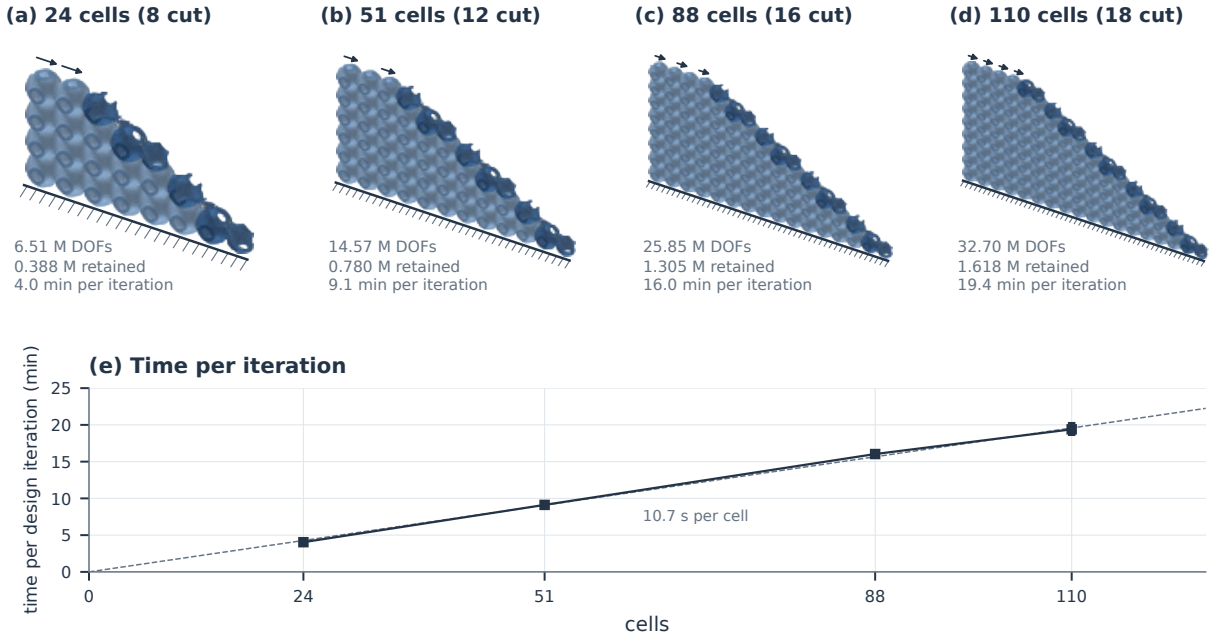
Figure 16: Plates of the scale demonstration. (a–d) Plates of 24, 51, 88 and 110 cells with the proportions and cut of the plate in Figure 15, at the uniform start \tau = 0.40 , drawn to the same scale. Each plate stands on its clamped long side (hatched), and the opposite face carries an in-plane traction along the long side (arrows). Light: uncut cells; dark: cut cells. Each panel gives the DOFs of the cut finite-element model, the free retained DOFs and the mean time per design iteration. (e) Time per design iteration against the number of cells (squares: mean; bars: range over the timed iterations). The dashed line is proportional to the number of cells, with the mean time of 10.7 s per cell. Memory use is given in Supplementary Table ST20.
