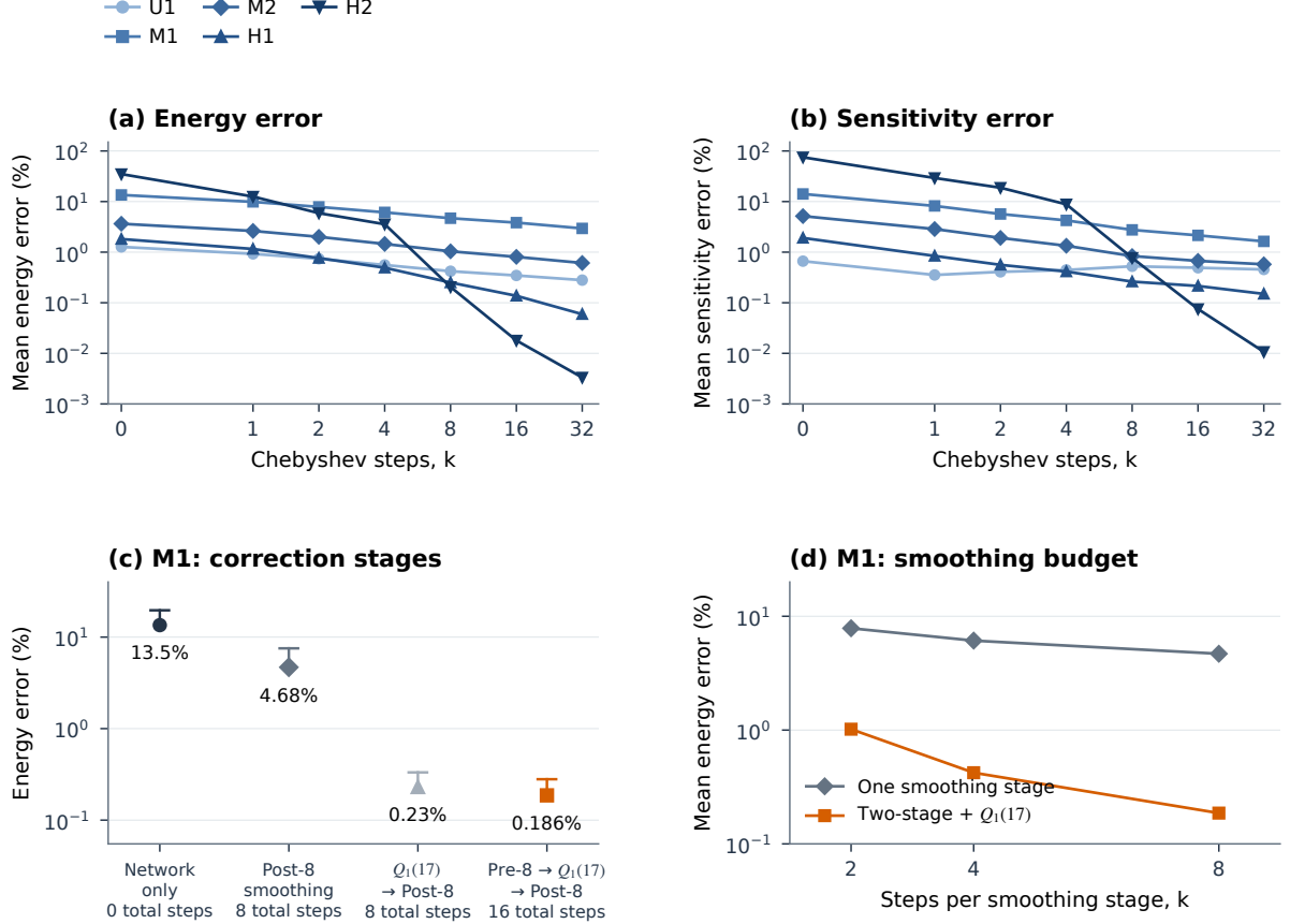
Figure 8: Correction of the base network with fixed network parameters. (a,b) Mean energy error and sensitivity error during Chebyshev smoothing on five cells. (c) M1 without correction, with eight smoothing steps, with a coarse-grid correction followed by eight steps, and with eight steps on each side of the coarse-grid correction; dots show means and caps the 90th percentile. (d) M1: mean energy error against the number k of steps per smoothing stage, for a single smoothing stage and for the cycle of k pre-smoothing steps, the Q_1(17) coarse-grid correction and k post-smoothing steps. All panels use traction loads, fixed retained displacements and a = b/30 . In (a,b) the step axis is linear from zero to one and logarithmic thereafter.
