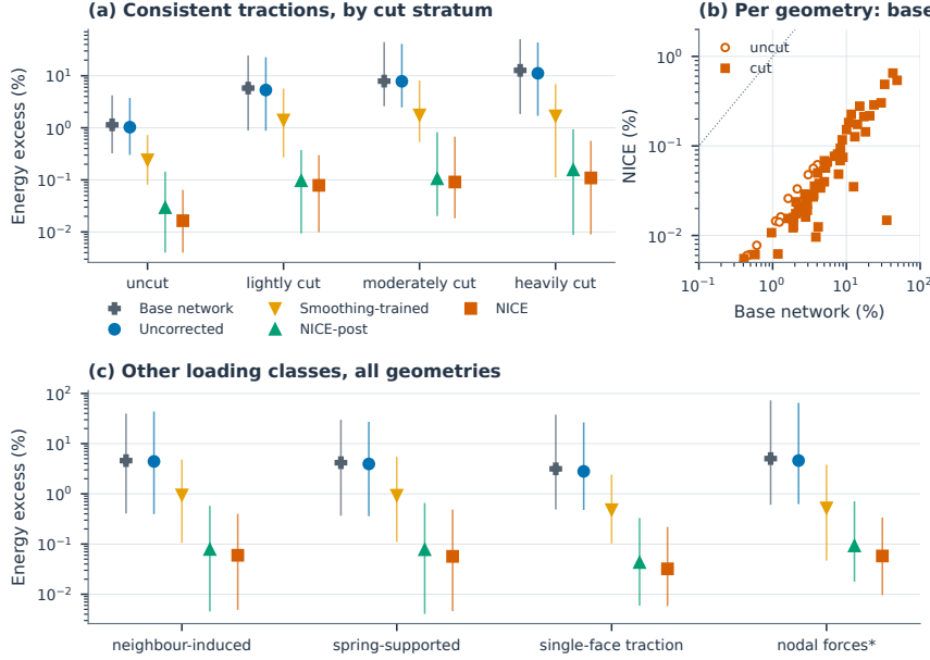
Figure 5: Directional energy error of the learned substructures on the 80 validation geometries. Each observation is a geometry's mean directional energy excess q^T(\hat{S} - S)q/(q^T S q) over the validation directions of a loading class. (a) Consistent tractions, 20 geometries per cut stratum: markers give the mean over geometries and bars the range from the 10th percentile to the maximum. (b) Geometry means of the base network and of NICE under consistent tractions, open markers for uncut and filled markers for cut geometries; the dotted line denotes equality. (c) Neighbour-induced retained displacements, stiffness-scaled spring supports, single-face consistent tractions and equal nodal forces (75 geometries for the first two classes, 80 for the others); the asterisk marks the nodal-force stress test. Twenty geometries (6 uncut, 14 cut) entered weight selection. Predictors as in Table 2.
