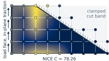
(a) Final NICE design
