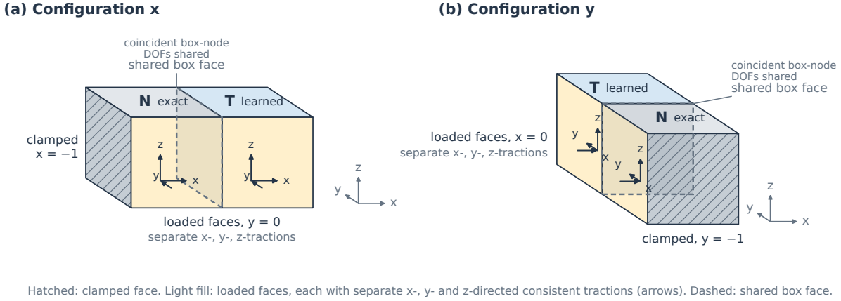
Figure 8: Supports and loading of the two-cell examples. (a) Configuration x: the neighbour is translated by (-1, 0, 0) , the face x = -1 is clamped, and face tractions act at y = 0 . (b) Configuration y: the translation is (0, -1, 0) , the face y = -1 is clamped, and tractions act at x = 0 . Each target (T) and neighbour (N) face carries separate x-, y- and z-directed consistent-traction loads. Coincident box-node DOFs are shared across the interface; non-box cut-band DOFs remain local. Cut targets also receive three cut-surface tractions, analysed separately.
