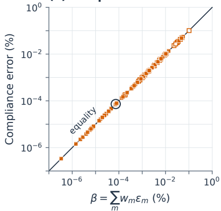
(a) Compliance error follows \beta
