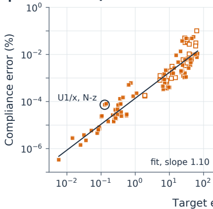
(b) Compliance error follows w
