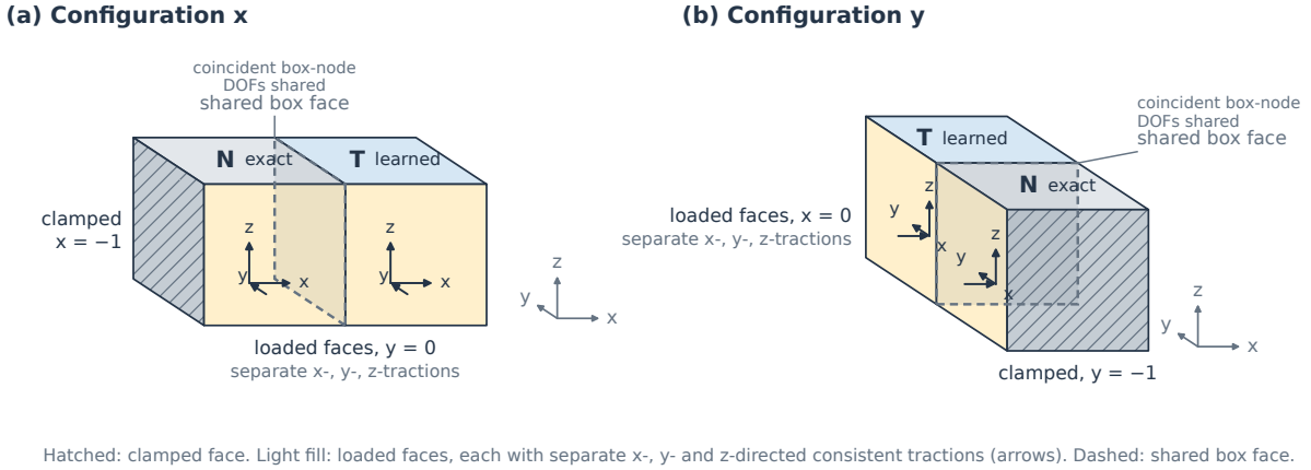
Figure 8: Supports and loading of the two-cell assemblies. (a) Configuration x: the neighbour is translated by (-1, 0, 0) , the face x = -1 is clamped, and face tractions act at y = 0 . (b) Configuration y: the translation is (0, -1, 0) , the face y = -1 is clamped, and tractions act at x = 0 . Each target (T) and neighbour (N) face carries separate x-, y- and z-directed consistent-traction loads. Coincident box-node DOFs are shared across the interface; non-box cut-band DOFs remain local. Cut targets also receive three cut-surface tractions, analysed separately.
