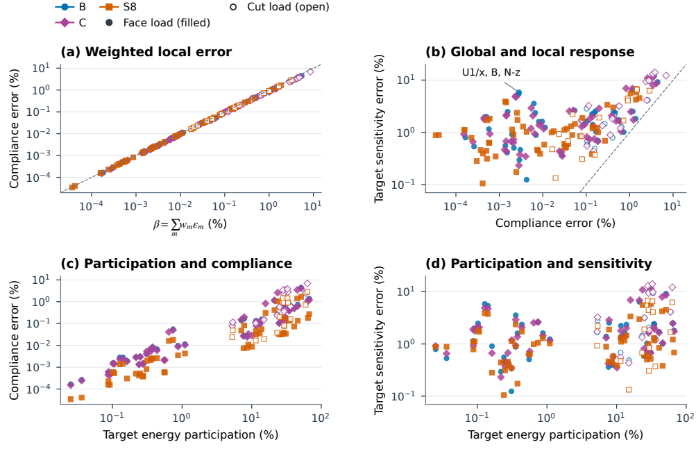
Figure 10: Participation-weighted compliance error and local sensitivity. Each point is one load for one model-configuration combination: 192 observations from the 25 model-configuration combinations in Figure 9. Filled markers denote face loads and open markers macro-cut loads. (a) Compliance error against \beta = \sum_m w_m \varepsilon_m , with w_m = q_m^T S_m q_m / C and \varepsilon_m = q_m^T (\hat{S}_m - S_m) q_m / (q_m^T S_m q_m) , evaluated at the exact assembled retained displacement. Only the learned target contributes to \beta . (b) Compliance and target-cell sensitivity errors under the same loads; the annotation identifies B on U1/x under the neighbour-z load. Dashed lines in (a,b) denote equality. (c,d) The two response errors versus the target's exact energy participation.
