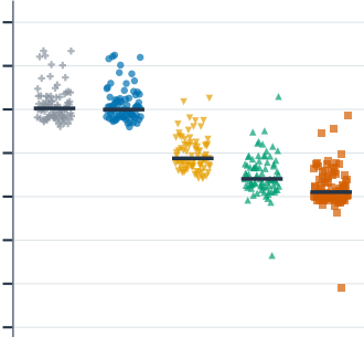
(c) Single-face point loads
