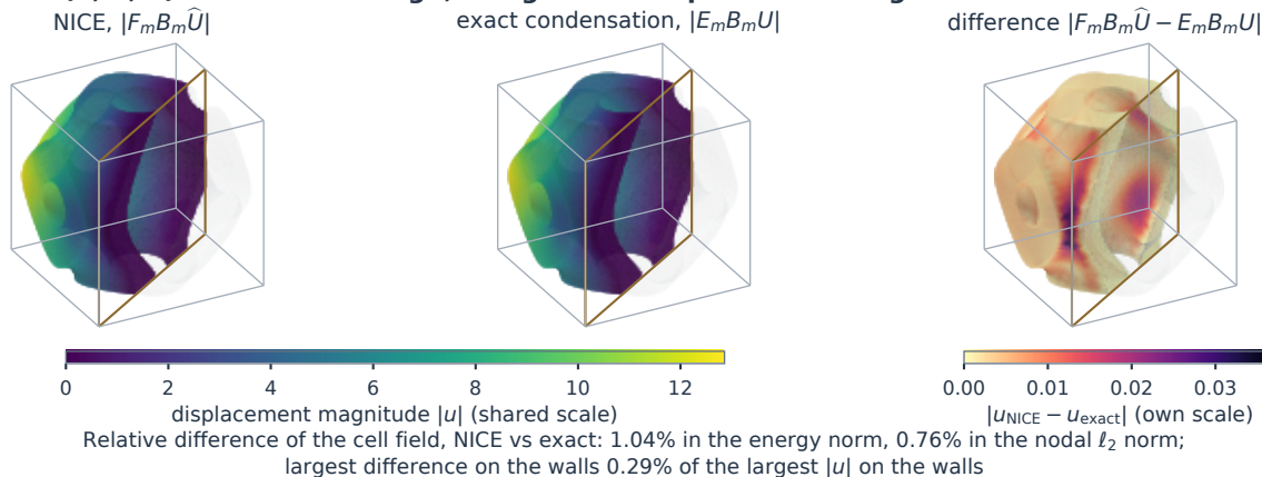
(c) Cut cell (3, 2, 0) at the final design, design load: displacement magnitude on the walls
