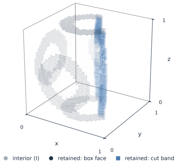
(a) Retained and interior DOFs
