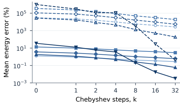
(a) Traction: energy
