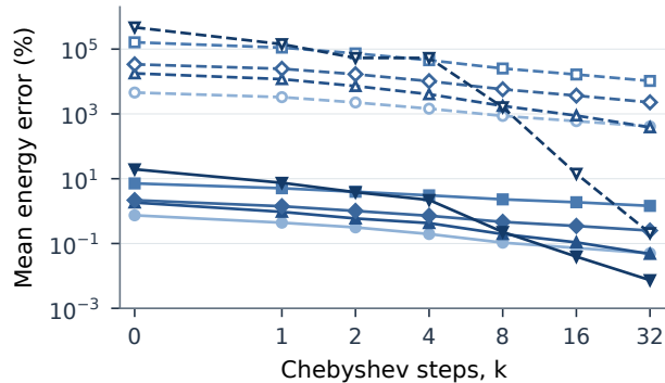
(b) Nodal force: energy
