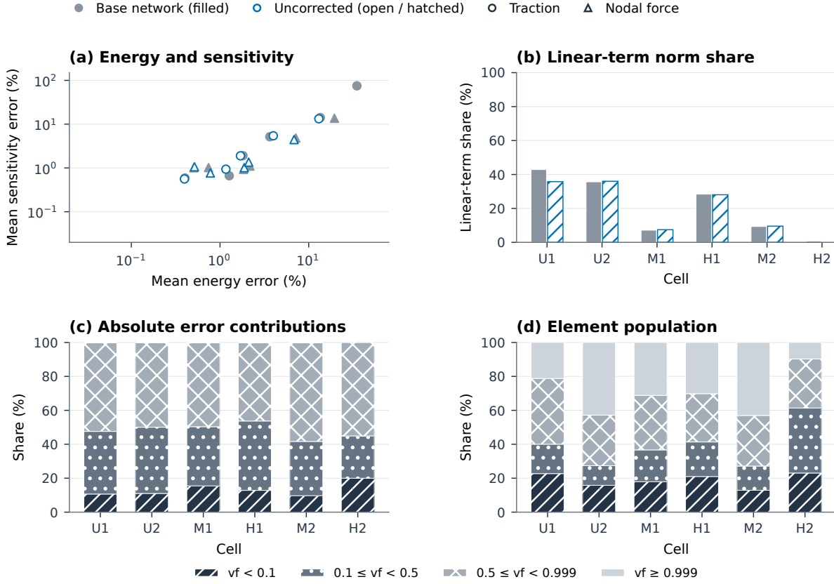
Figure S03: Field-based sensitivity-error diagnostics. (a) Paired mean energy and sensitivity errors for consistent-traction and nodal-force responses, using six cells of the base network and five of Uncorrected. (b) Consistent-traction linear-term norm share \|D_1\|_F / (\|D_1\|_F + \|D_2\|_F) , where D_1 + D_2 is the sensitivity-error matrix over all eight design components and evaluated directions. (c,d) Shares of absolute elementwise sensitivity-error contributions and element counts in four mutually exclusive material-volume-fraction groups for the base network under consistent tractions. Each error group sums absolute contributions over its elements, design components and directions before normalisation by the total. Filled markers identify the base network and open markers and hatched bars in (a,b) Uncorrected; Uncorrected is shown for U1, U2, M1, H1 and M2 (Table ST05a).
