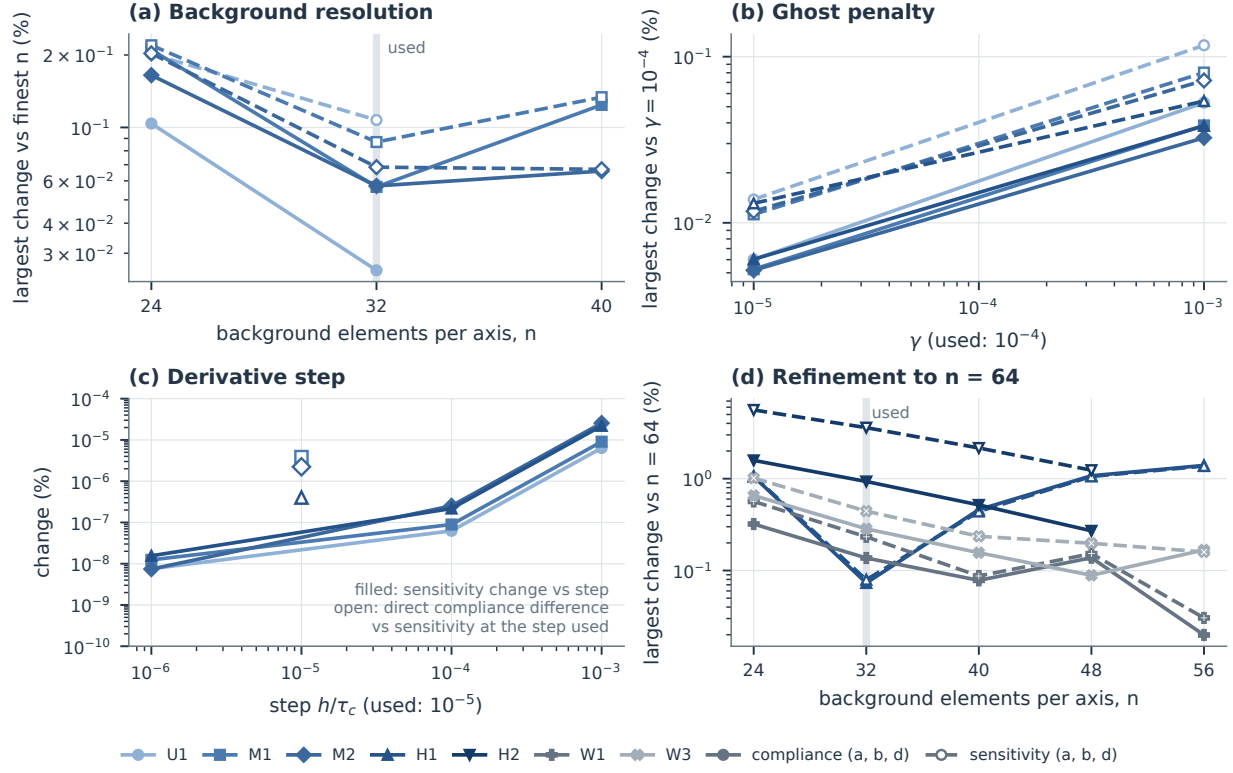
Figure S01: Verification of the CutFEM reference. Single cells clamped on one box face and loaded by unit consistent tractions on another face in the three Cartesian directions. In (a), (b) and (d), solid lines with filled markers give the compliance and dashed lines with open markers the thickness sensitivity, each as the largest relative change over the three loads. (a) Change against the finest background resolution computed for U1 ( n = 40 ) and for M1 and M2 ( n = 48 ); the reference used throughout has n = 32 . (b) Change when the ghost-penalty coefficient is varied from the value 10^{-4} used throughout. (c) Filled: largest relative change of the sensitivity when the finite-difference step of the moment derivatives is varied from the value h_c = 10^{-5}\tau_c used throughout, at most 2.6 \times 10^{-5}\% at 10^{-3}\tau_c and a hundredfold smaller at 10^{-4}\tau_c ; open: largest relative difference between central compliance differences and the sensitivity at the step used. (d) Refinement to n = 64 of H1, H2 and the validation cells with the largest NICE error (W1) and the thinnest walls (W3), the data of Table ST10; H2 has no n = 56 solution.
