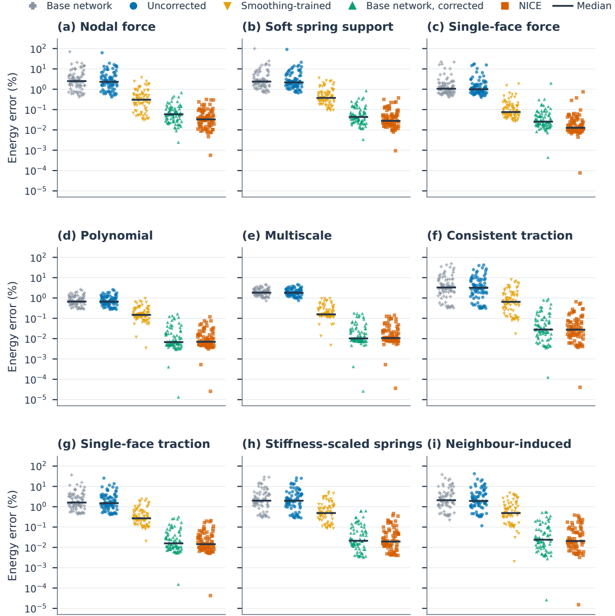
Figure S02: Distributions of geometry-level directional energy errors. Each point is one validation geometry's mean directional energy error in the identity orientation; horizontal bars are population medians. The nodal-force, spring-support, single-face-force, polynomial, multiscale, consistent-traction and single-face consistent-traction classes contain 80 geometries, and the stiffness-scaled support and neighbour-induced displacement classes 75, the same populations as Table ST03. The five variants of Table ST03 (base network, Uncorrected, Smoothing-trained, base network with the correction applied at deployment, NICE) use the markers and colours of the main-text figures; deterministic horizontal offsets separate overlapping observations. All panels share the logarithmic error axis.
