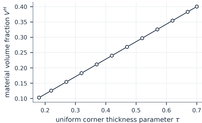
(b) Material volume fraction
