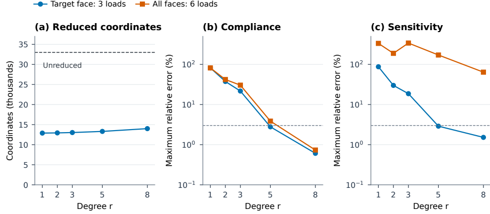
Figure 11: Response errors caused by restricting box-face displacements. Both cells of H1/x use exact operators and Bernstein degree r on every box face, with unrestricted non-box cut-band DOFs. (a) Number of retained DOFs; the dashed line denotes the 32,991 DOFs of the full representation. (b,c) Maximum compliance and target-cell sensitivity errors over the three target-face loads or all six target- and neighbour-face loads; cut-surface tractions are excluded. Errors are relative to the full retained-space solution; horizontal lines mark 3%.
