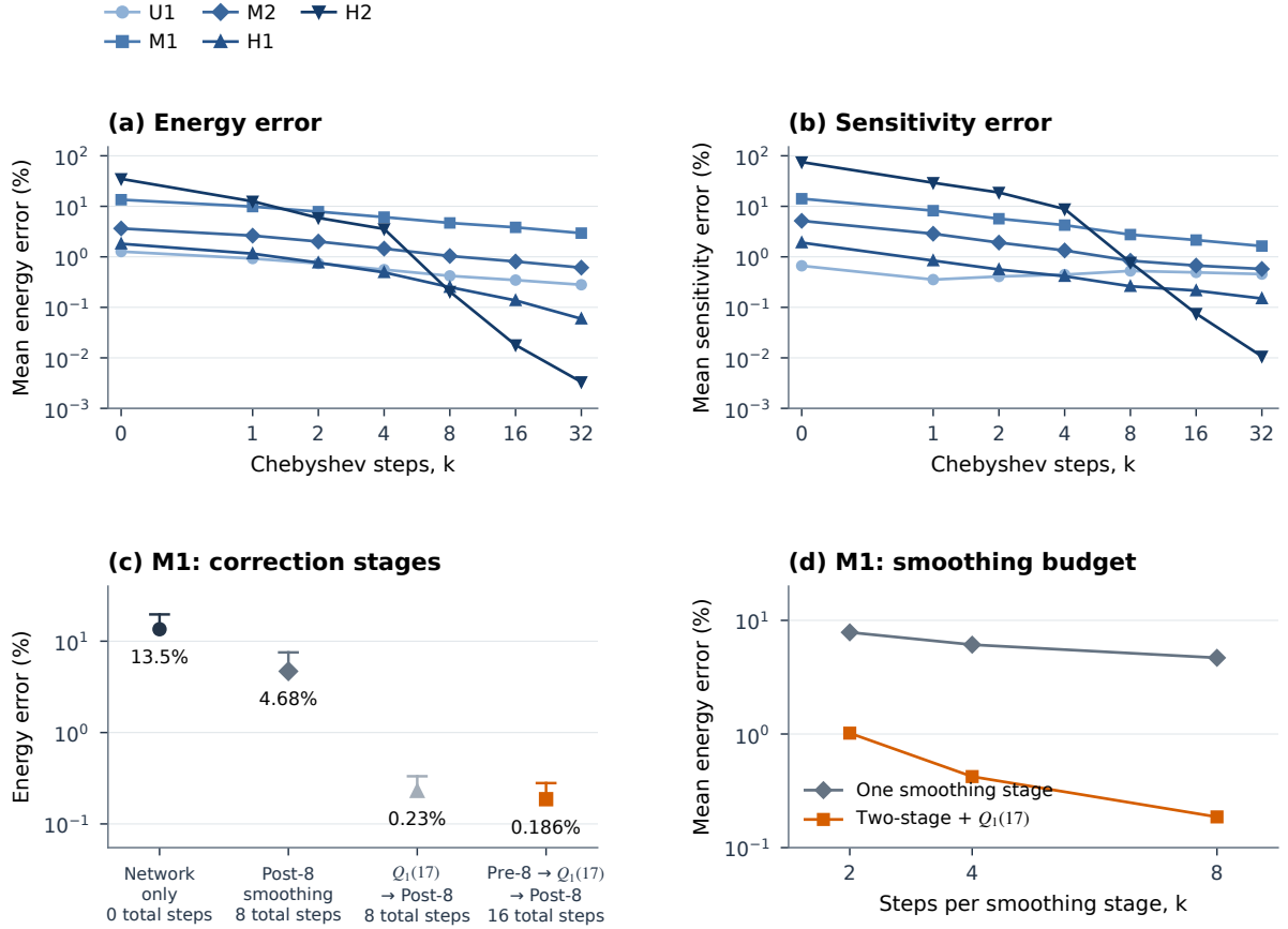
Figure 8: Accuracy gained by correcting the base network at fixed network parameters. (a,b) Mean directional energy error and field-based sensitivity error during Chebyshev smoothing on five cells. (c) M1 with no correction, eight smoothing steps, coarse-grid correction followed by eight steps, and eight steps on each side of the coarse-grid correction; dots show means and caps the 90th percentile. (d) M1: mean energy error against the number k of steps per smoothing stage, for one smoothing stage alone and for k pre-smoothing steps, the Q_1(17) coarse-grid correction and k post-smoothing steps. All panels use consistent tractions, fixed retained displacements and a = b/30 ; in (a,b) the step axis is linear from zero to one and logarithmic thereafter.
