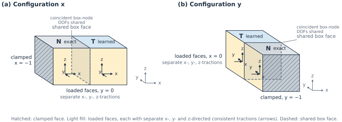
Figure 4: Supports and loading of the two-cell examples. (a) Configuration x: the neighbour is translated by (-1, 0, 0) , the face x = -1 is clamped, and face tractions act at y = 0 . (b) Configuration y: the translation is (0, -1, 0) , the face y = -1 is clamped, and tractions act at x = 0 . Each target (T) and neighbour (N) face carries separate x-, y- and z-directed consistent-traction loads. Coincident box-node DOFs are shared across the interface; non-box cut-band DOFs remain local. Cut targets also receive three cut-surface tractions, analysed separately.
