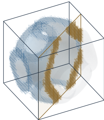
(b) Cut cell next to the support
