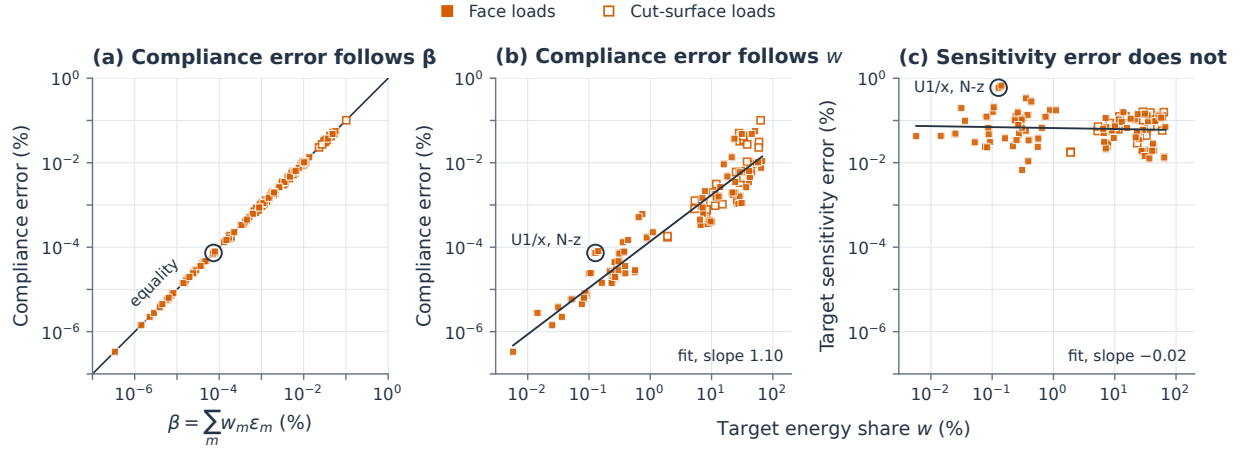
Figure 11: The target's energy share scales down the compliance error but not the sensitivity error. NICE in the fourteen configurations of the seven selection cells, one point per load: 84 face loads (filled markers) and 30 cut-surface loads (open markers); the maxima over the loads are given in Tables ST08 and ST09. (a) Compliance error against \beta = \sum_m w_m \varepsilon_m , with the energy shares w_m = q_m^T S_m q_m / C and energy errors \varepsilon_m = q_m^T (\hat{S}_m - S_m) q_m / (q_m^T S_m q_m) , evaluated at the exact assembled retained displacement; only the learned target contributes to \beta . The line denotes equality. For every load the compliance error lies between 0.963 and 1.004 times \beta ; the five ratios above 1 correspond to at most 7.8 \times 10^{-10} of the compliance, whereas the residual work of the pair solves reaches 1.8 \times 10^{-8} of the compliance (Supplementary Note S4.3). (b) Compliance error and (c) target-cell sensitivity error against the target's exact energy share w ; solid lines are least-squares fits in logarithmic coordinates. The circled load is U1/x under the neighbour-face z traction (Table 5). The other four variants are shown in Figure S04.
