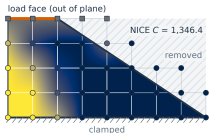
(c) Final design B2
