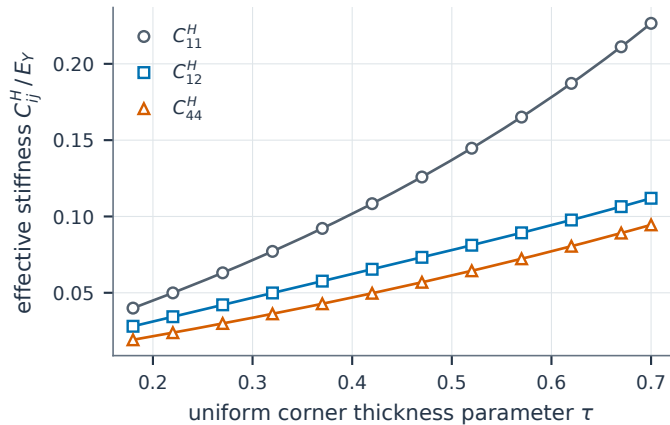
(a) Effective elasticity tensor (cubic)
