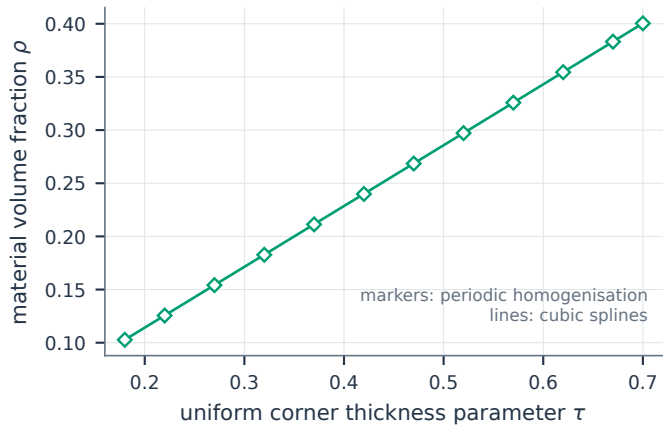
(b) Material volume fraction
