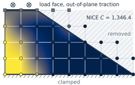
(a) Final design B2
