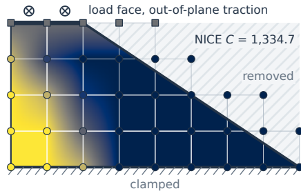
(b) Final design X-z
