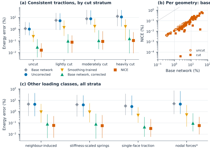
Figure 5: Directional energy error of the learned substructures on the 80 validation geometries. Each observation is a geometry's mean directional energy error q^T(\hat{S} - S)q/(q^T S q) over the validation directions of a loading class. (a) Consistent tractions, 20 geometries per cut stratum: markers give the mean over geometries and bars the range from the 10th percentile to the maximum. (b) Geometry means of the base network and of NICE under consistent tractions, open markers for uncut and filled markers for cut geometries; the dotted line denotes equality. (c) Neighbour-induced retained displacements, stiffness-scaled spring supports, single-face consistent tractions and equal nodal forces (75 geometries for the first two classes, 80 for the others); the asterisk marks the nodal-force stress test. Twenty geometries (6 uncut, 14 cut) were used for model selection. Variants as in Table 2 and the note below it; 'Base network, corrected' is the base network with the correction applied at deployment.
