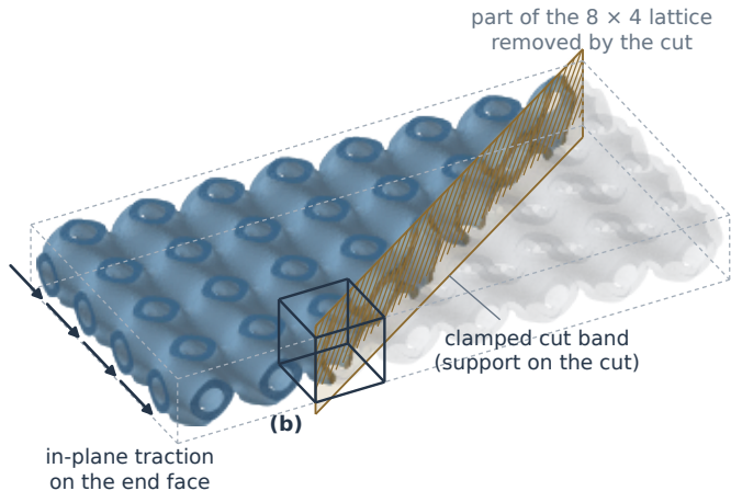
(a) A lattice trimmed to a part: cut cells carry the support
