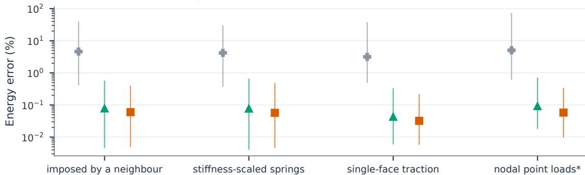
(c) Other load classes, all cells
