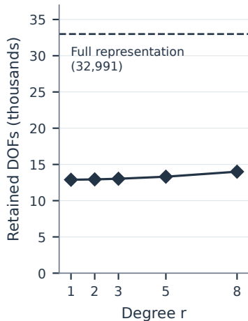
(a) Retained DOFs
