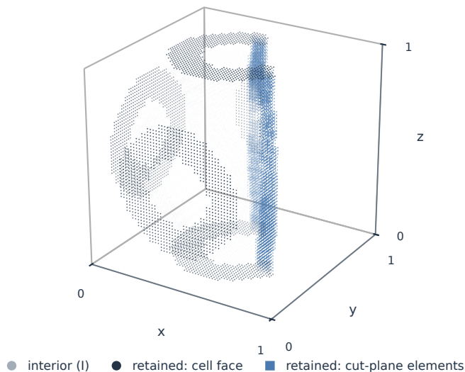
(a) Retained and interior DOFs
