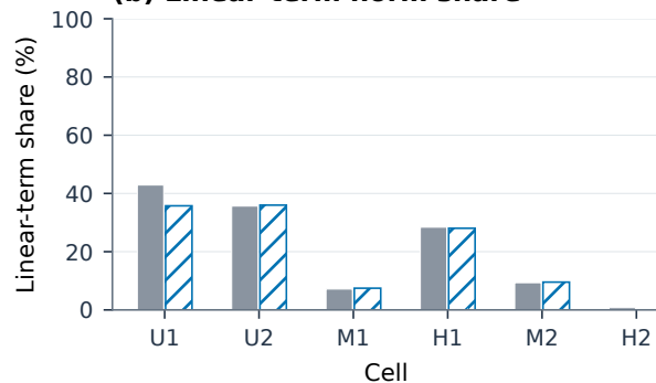
(b) Linear-term norm share
