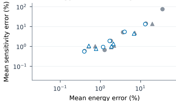
(a) Energy and sensitivity
