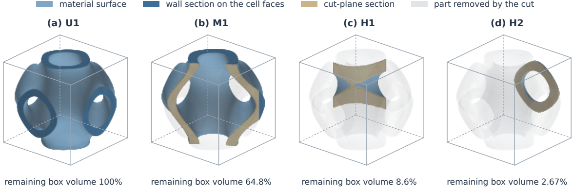
Figure 4: Representative validation geometries. (a) Uncut cell U1, (b) moderately cut cell M1 and (c,d) heavily cut cells H1 and H2, shown at the same unit-box scale and from the same viewing direction. Light blue shows the material surface, dark blue the wall section on the cell faces and sand the section on the cut plane. The part removed by the cut is drawn in translucent grey, and the cells are viewed from the side of the cut. The percentages give the box volume that remains after the cut, relative to the unit box, before the intersection with the thin-wall material. The surfaces are reconstructed from Eq. (1) on a grid of 129 points per axis and serve only for visualisation.
