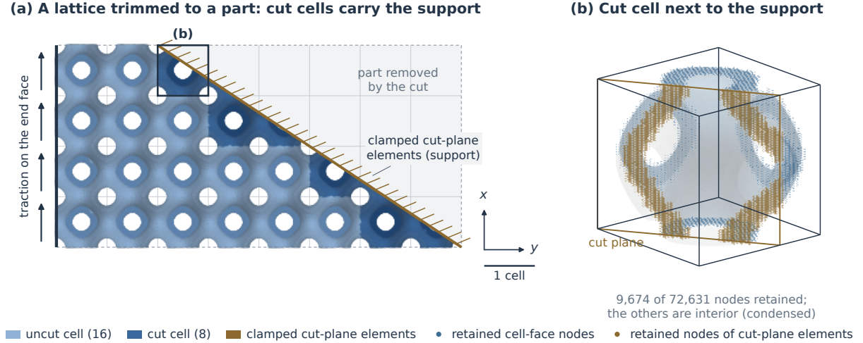
Figure 1: A lattice trimmed to the shape of a part, whose cut cells carry the support. (a) Plan view of a single layer of 8 \times 4 Schwarz-P cells (Eq. (1), uniform \tau = 0.40 ) trimmed by a plane. The layer has 16 uncut cells (light) and eight cut cells (dark); the part removed by the cut is drawn pale with a dashed outline. The plate is clamped at its cut: every degree of freedom of the cut-plane elements of every cut cell is fixed (hatched line). The end face carries an in-plane traction load of unit resultant (arrows). (b) The cut cell outlined in (a), with translucent walls and the cut plane. Of the 72,631 nodes of its Q_2 model, the 9,674 nodes on the cell faces (blue) and in the cut-plane elements (sand) are retained. All other nodes are interior and are eliminated by static condensation. The surfaces are reconstructed from Eq. (1) for visualisation only.
