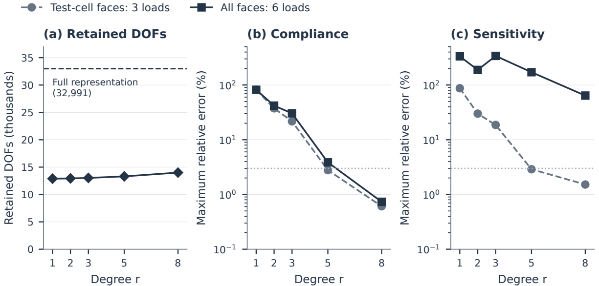
Figure 12: Response errors caused by restricting the cell-face displacements. Both cells of H1/x use their exact condensed stiffness and Bernstein polynomials of degree r on every cell face. The DOFs of the cut-plane elements that do not lie on the cell faces remain unrestricted. (a) Number of retained DOFs; the dashed line marks the 32,991 DOFs of the full representation. (b,c) Maximum compliance error and maximum test-cell sensitivity error, over the three loads on the test-cell face or over all six loads on the test-cell and neighbour faces. Traction loads on the cut surface are excluded. Errors are relative to the solution with all retained DOFs, and the horizontal lines mark 3%.
