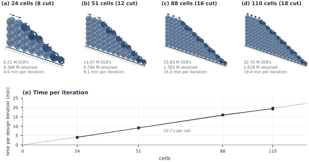
Figure 16: Plates of the scale study. (a–d) Plates of 24, 51, 88 and 110 cells with the proportions and cut of the plate in Figure 15, at the uniform start \tau = 0.40 , drawn to the same scale. Each plate stands on its clamped long side (hatched), and the opposite face carries an in-plane traction along the long side (arrows). Light: uncut cells; dark: cut cells. Each panel gives the DOFs of the cut finite-element model, the free retained DOFs and the mean time per design iteration. (e) Time per design iteration against the number of cells (squares: mean; bars: range over the timed iterations). The dashed line is proportional to the number of cells, with the mean time of 10.7 s per cell. Memory use is given in Supplementary Table ST20.
