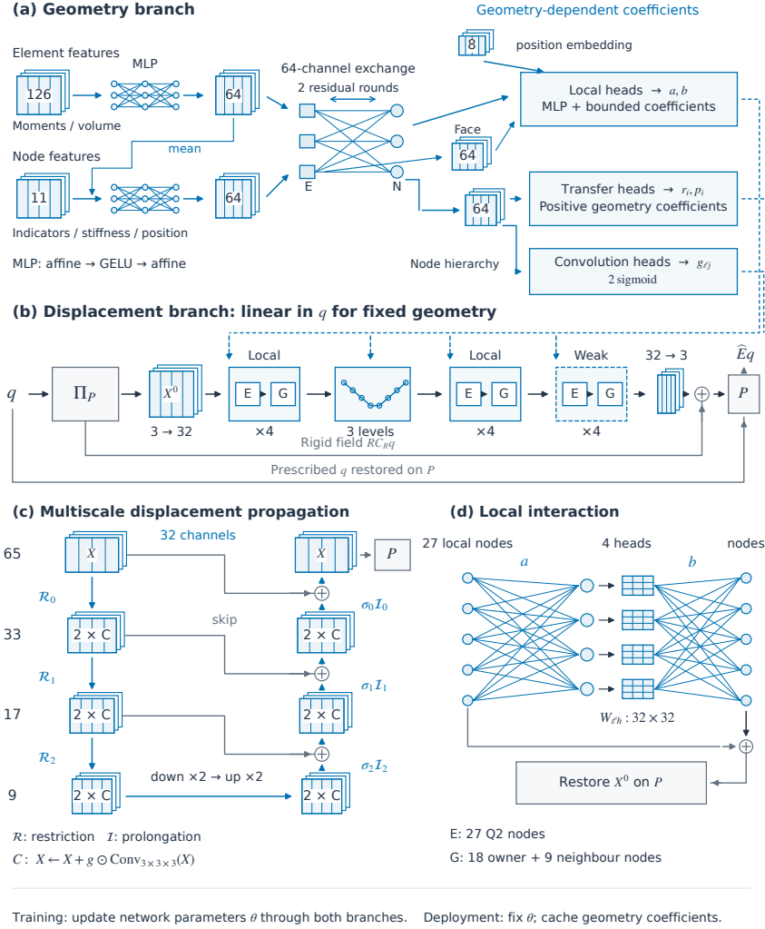
Figure 3: Architecture of the network for the interior displacements. (a) Geometry branch. Element and node encoders produce geometry feature vectors with 64 channels, which then exchange information in two residual rounds. Coefficient heads compute from these vectors the coefficients of the local interactions, the grid transfers and the convolutions. The heads of the local interactions also receive a position embedding, which identifies the local node position within a stencil (Appendix G.1). (b) Displacement branch. The retained displacements, with their rigid-body part removed, pass through four pairs of local interactions, the grid hierarchy, four further pairs and four pairs on stencils that contain weakly connected nodes (labelled 'Weak'). Linear maps convert the three displacement components to 32 feature channels at the input and back at the output. Bypass paths without learned parameters reconstruct the rigid-body motion and restore the prescribed retained displacements. (c) Multiscale displacement propagation. Restriction \mathcal{R} and prolongation \mathcal{I} connect the grids of the hierarchy, which have 65, 33, 17 and 9 background positions per axis. Each coarse grid applies two residual convolutions on the downward pass and two on the upward pass. (d) Local interaction. The features at the 27 local nodes of a stencil are gathered with geometry-dependent weights into four heads, and the channels are mixed within each head. The result is scattered back to the nodes and added to the incoming features, and the retained features are then restored. E and G denote element and ghost-face interactions. Blue dashed arrows carry geometry-dependent coefficients, and solid arrows carry features or displacements. For fixed geometry, the complete displacement path is linear.
