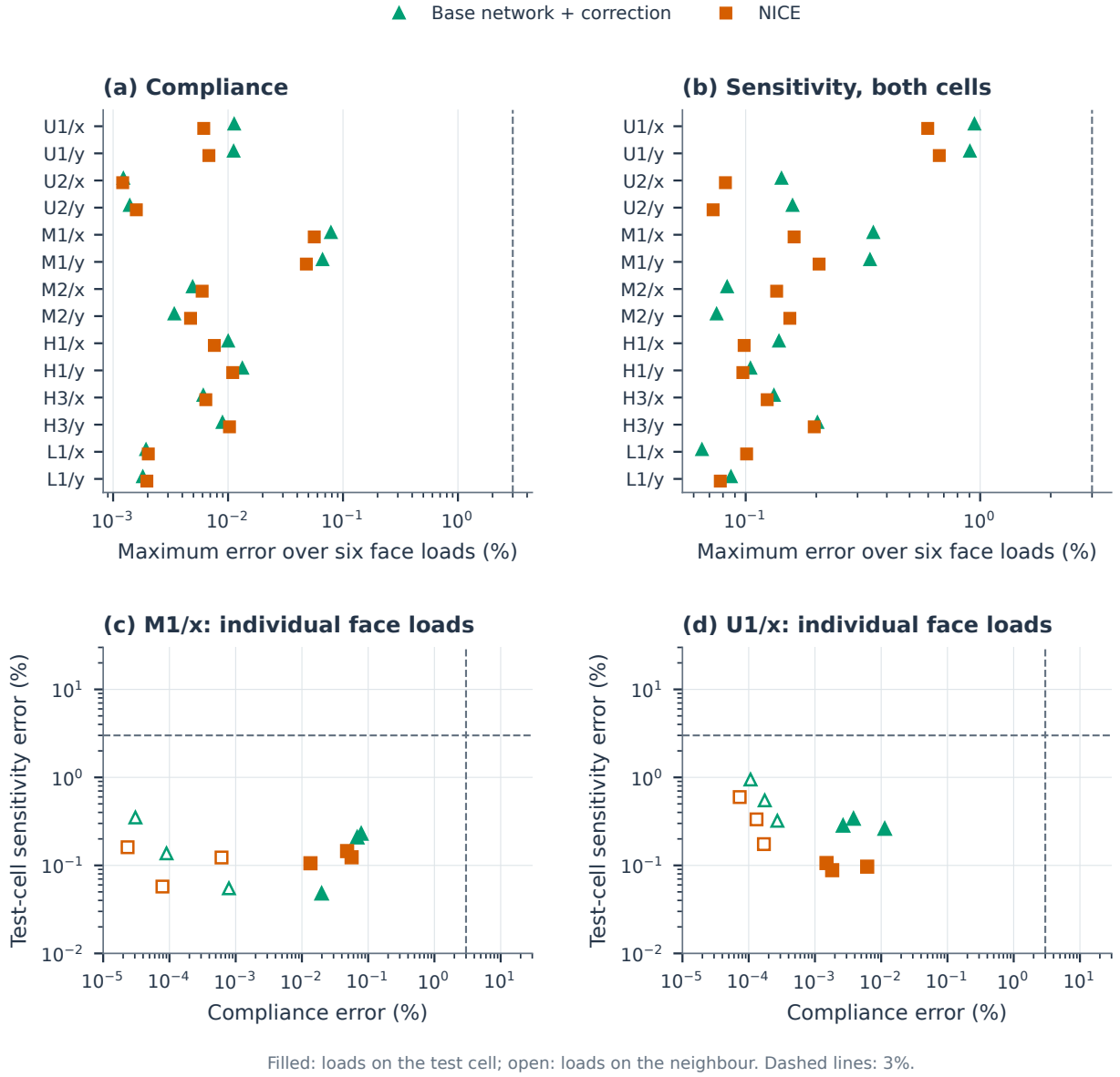
Figure 10: Compliance and thickness sensitivity in two-cell assemblies. The test cell is represented by a learned substructure and the neighbouring cell by exact static condensation. The figure shows NICE and Base network + correction, which is the base network with the correction applied at deployment, without retraining. (a,b) Maximum errors over the six face loads in each configuration; the sensitivity error is also maximised over both cells. (c,d) Compliance error and test-cell sensitivity error under each face load on M1/x and U1/x. Filled markers denote loads on the face of the test cell, and open markers loads on the face of the neighbouring cell. Dashed lines mark 3%. Supplementary Table ST08 gives all results. It also includes the base network and the two variants of Supplementary Note S8. None of these three variants was evaluated in every configuration.
