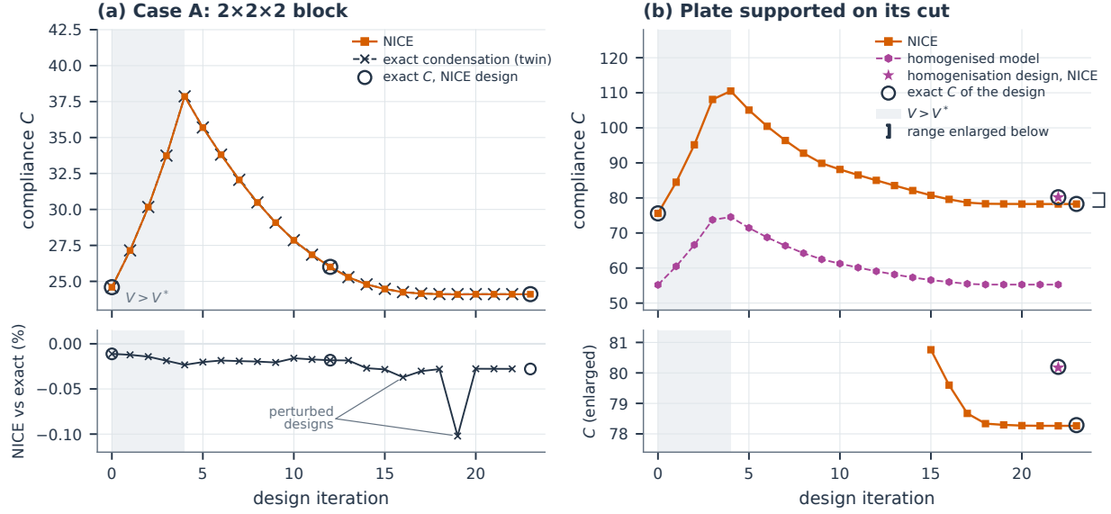
Figure 14: Thickness optimisation with NICE. (a) Case A: compliance histories of the NICE optimisation and of the twin optimisation with exact static condensation. Open circles give the exact compliance of the NICE designs at iterations 0, 12 and 23. The compliance first rises while the volume is reduced from 1.25V^* to V^* (shading, iterations 0–3). Lower strip: NICE compliance relative to the twin run at the same design iteration (line) and relative to the exact compliance of the same design (circles: -0.011\% , -0.018\% , -0.028\% ). The designs of the two runs coincide at iterations 0–4 and differ afterwards. At iterations 16 and 19, labelled 'perturbed designs', the NICE design had been perturbed by the fallback of the geometry generator (Supplementary Table ST19a). (b) Plate supported on its cut. The curves show the NICE compliance from the uniform start and the compliance of the homogenised macroscale model along its own optimisation (dashed line). The star marks the homogenisation design analysed with NICE on the cut geometry, placed at the last macroscale iteration. Open circles give the exact compliance of the uniform start, the final NICE design and the homogenisation design. Shading: design iterations with V > V^* . Lower strip: the range marked by the bracket, enlarged, from iteration 15.
