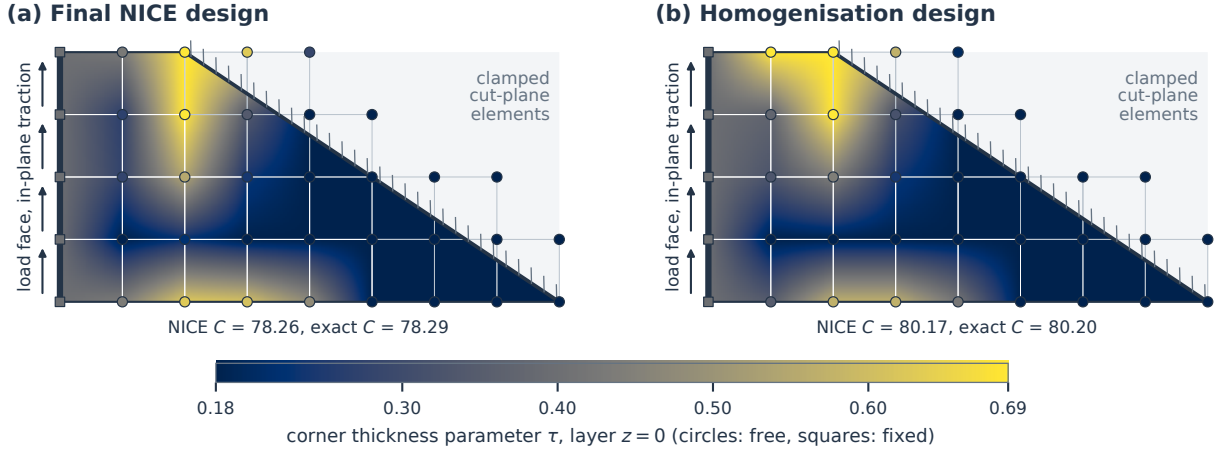
Figure 15: Designs of the plate supported on its cut. (a,b) Corner thickness parameters of the final NICE design and of the homogenisation design in the layer z = 0 , drawn with the long side horizontal. Circles denote design variables, and squares denote the fixed vertices in the plane of the loaded face. Vertices drawn in the removed region are corners of cut cells. The thick hatched line marks the clamped cut-plane elements, and the arrows mark the loaded face and the direction of the in-plane traction. The compliances in (a,b) are the NICE and exact values of the same design (Supplementary Table ST21).
