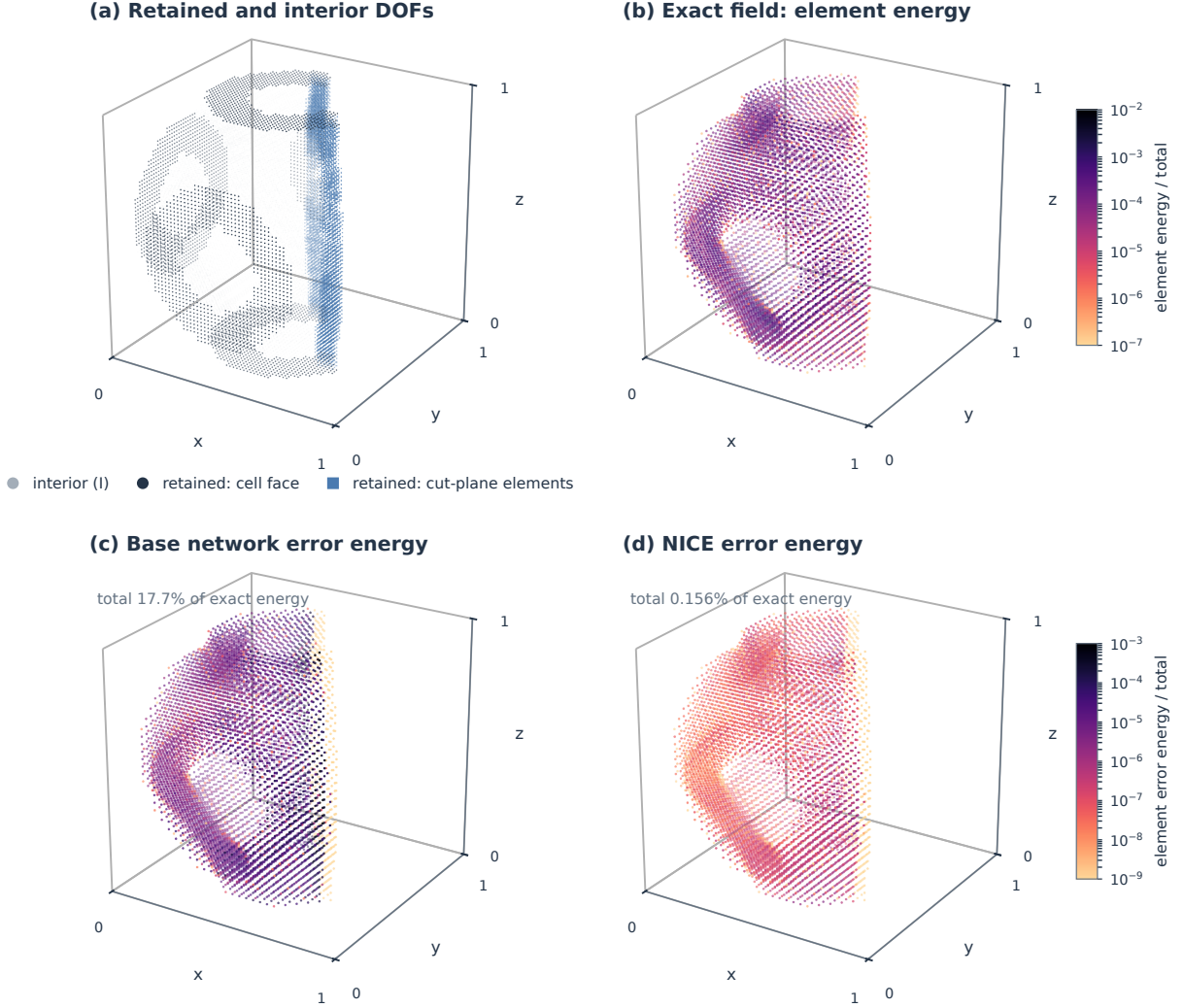
Figure 7: Retained DOFs and spatial distribution of the interior displacement error in M1. (a) Retained DOFs on the cell faces, retained DOFs of the cut-plane elements, and interior DOFs. (b) Bulk element energies of the exact field for one traction-load test displacement, relative to its total energy. (c,d) Bulk element energies of the error of the base network and of NICE for the same retained displacements, relative to the total energy of the exact field in (b), on a common colour scale. The cut-plane elements carry no error because their DOFs are retained.
