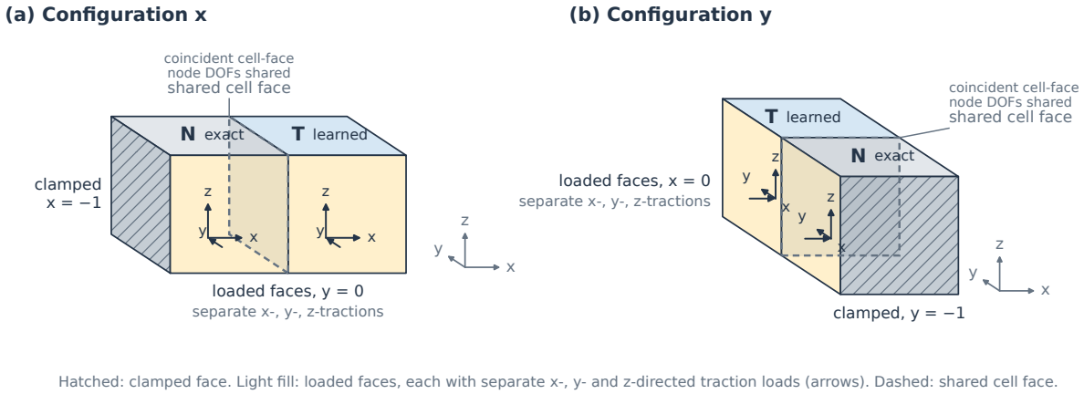
Figure 9: Supports and loads of the two-cell assemblies. (a) Configuration x: the neighbouring cell is translated by (-1, 0, 0) , the face x = -1 is clamped, and the traction loads act on the faces at y = 0 . (b) Configuration y: the translation is (0, -1, 0) , the face y = -1 is clamped, and the traction loads act on the faces at x = 0 . The loaded faces of the test cell (T) and of the neighbouring cell (N) each carry separate traction loads in the x, y and z directions. The coincident DOFs of the cell-face nodes are shared across the interface, and the DOFs of cut-plane elements that do not lie on the cell faces remain local to their cell. Cut test cells also carry three traction loads on the cut surface, which are analysed separately.
