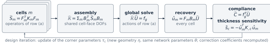
Figure 2: Overview of NICE: condensed stiffness of one cell, assembly and design. (a) The rigid-body part of the retained displacements is separated before the network predicts the interior displacements, so that the network acts only on the deformation. The rigid-body field is then added back and the prescribed retained displacements are restored, which gives \hat{E}q . The two-grid correction \mathcal{W} reduces the interior force imbalance with the retained displacements held fixed, which gives \hat{u} = Fq . Applying the cell stiffness K and then the transpose F^T gives the corresponding nodal forces on the retained DOFs, \hat{S}q . The ordering S \preceq \hat{S} \preceq \hat{S}_{\text{net}} in (a), where \hat{S}_{\text{net}} is the condensed stiffness without correction, is that of Proposition 2. This ordering concerns the energy error and does not apply to the sensitivity error. (b) The condensed stiffness matrices of the cells are assembled on the shared cell-face DOFs, and the assembled system is solved. The displacements of every cell are recovered from the assembled solution, and the compliance and the thickness sensitivity are computed. A design iteration updates the corner thickness parameters and therefore changes the geometry of every cell. The network parameters stay the same, and the coefficients of \mathcal{W} are recomputed.
