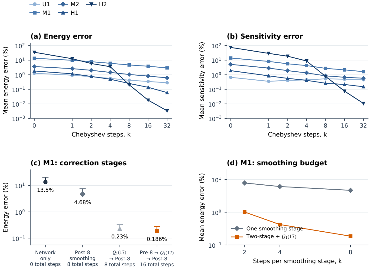
Figure 8: Correction of the base network with fixed network parameters. (a,b) Mean energy error and sensitivity error during Chebyshev smoothing on five cells. (c) M1 without correction, with eight smoothing steps, with a coarse-grid correction followed by eight steps, and with eight steps on each side of the coarse-grid correction; dots show means and caps the 90th percentile. (d) M1: mean energy error against the number k of steps per smoothing stage, for a single smoothing stage and for the cycle of k pre-smoothing steps, the Q_1(17) coarse-grid correction and k post-smoothing steps. All panels use traction loads, fixed retained displacements and a = b/30 . In (a,b) the step axis is linear from zero to one and logarithmic thereafter.
