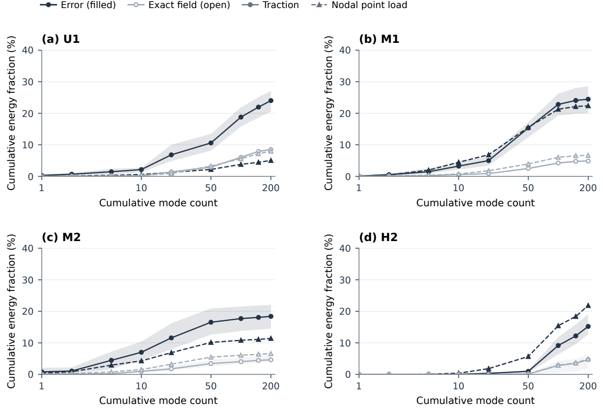
Figure 6: Spectral distribution of the interior displacement error of the base network. Panels show U1, M1, M2 and H2. The modes solve Av = \lambda Dv , with D = \text{diag}(A) , and are ordered by increasing eigenvalue. Filled dark markers denote the error and open light-grey markers the exact interior field. Solid lines with circles denote traction loads and dashed lines with triangles nodal point loads. Curves are means over the test displacements. Bands give the 10th to 90th percentiles over the test displacements under traction loads. Each cumulative fraction is normalised by the total interior energy of its own field or error.
