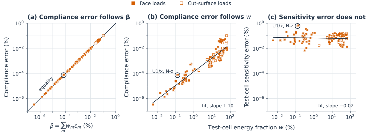
Figure 11: The energy fraction of the test cell scales down the compliance error but not the sensitivity error. Results of NICE in the fourteen configurations of the seven test cells, one point per load: 84 face loads (filled markers) and 30 cut-surface loads (open markers). Supplementary Tables ST08 and ST09 give the maxima over the loads. (a) Compliance error against \beta = \sum_m w_m \varepsilon_m , with the energy fractions w_m = q_m^T S_m q_m / C and the energy errors \varepsilon_m = q_m^T (\hat{S}_m - S_m) q_m / (q_m^T S_m q_m) evaluated at the exact assembled retained displacements. Only the learned test cell contributes to \beta . The line denotes equality. For every load, the compliance error lies between 0.963 and 1.004 times \beta . The five ratios above 1 correspond to an excess of at most 7.8 \times 10^{-10} of the compliance, whereas the residual work of the pair solves reaches 1.8 \times 10^{-8} of the compliance (Supplementary Note S4.3). (b) Compliance error and (c) test-cell sensitivity error against the exact energy fraction w of the test cell; solid lines are least-squares fits in logarithmic coordinates. The circled point is U1/x under the z traction load on the neighbour face. Figure S04 shows the corresponding results of the other variants.
