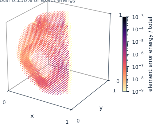
(c) Base network (uncorrected): error energy
