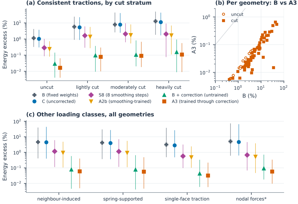
Figure 5: Directional energy error of the learned substructures on 80 unseen geometries. Each observation is a geometry's mean directional energy excess q^T(\hat{S} - S)q / (q^T S q) over the validation directions of a loading class. (a) Consistent tractions, 20 geometries per cut stratum: markers give the mean over geometries and bars the range from the 10th percentile to the maximum. (b) Geometry means of B and of the principal predictor A3 under consistent tractions; the dotted line denotes equality. (c) Neighbour-induced retained displacements, spring-supported faces, single-face consistent tractions and equal nodal forces, all available geometries (75 for the first two classes, 80 for the others); the nodal-force class is a stress test whose exact energy resides largely in the ghost penalty. Predictors as in Table 2.
