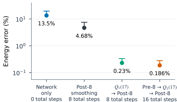
(c) M1: correction stages
