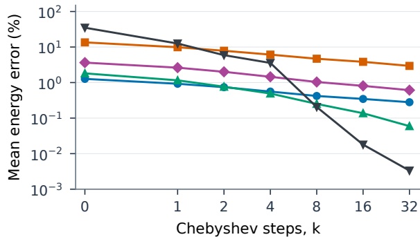
(a) Energy error
