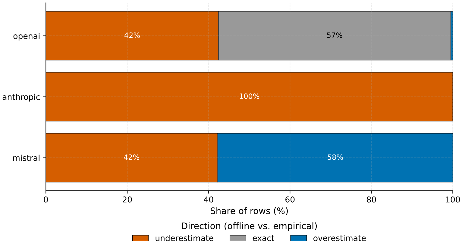
Direction of offline-tokenizer bias by provider
