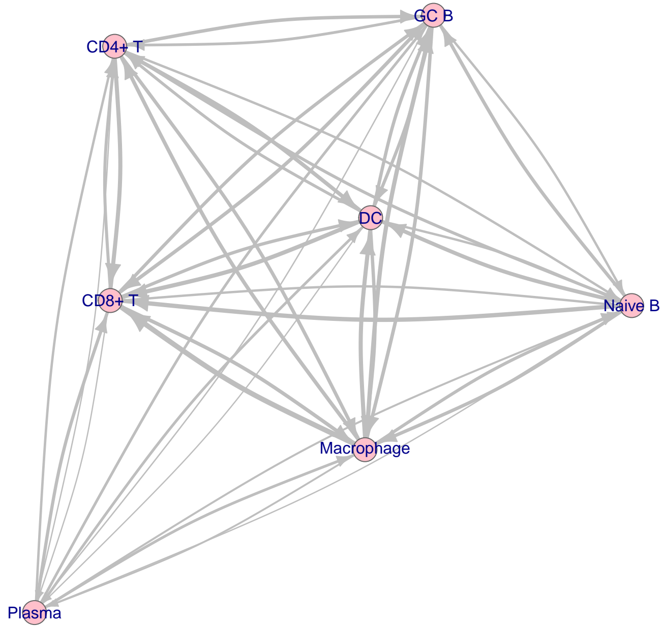
Directed cell-cell interaction network
