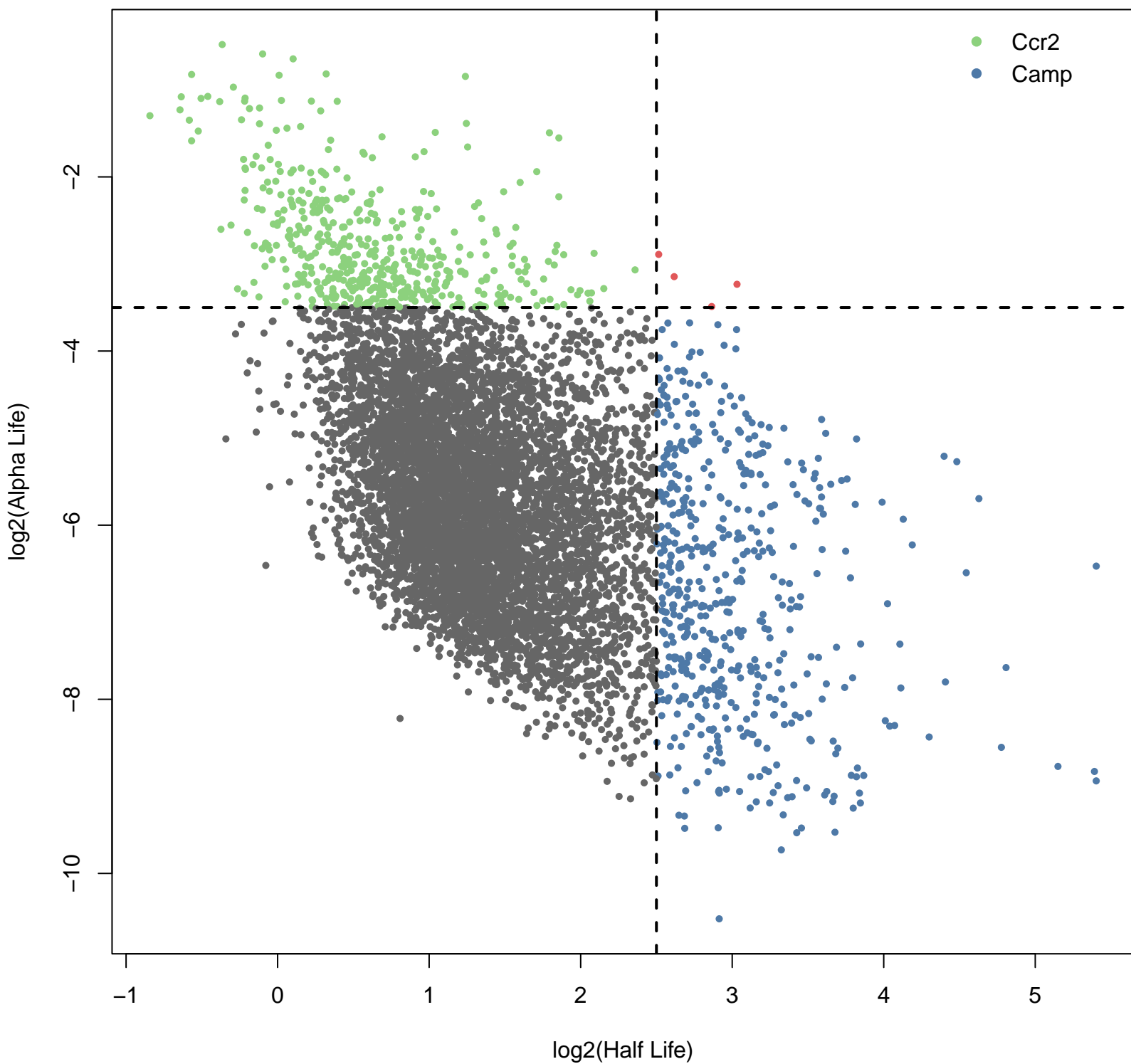
Half-life vs alpha-life scatter
