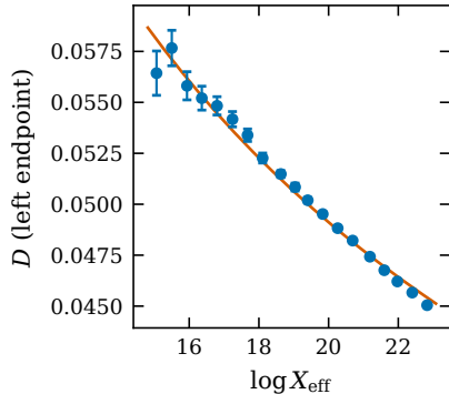
(c) \beta = 0.592
