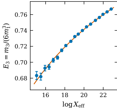
(b) \beta = 0.782
