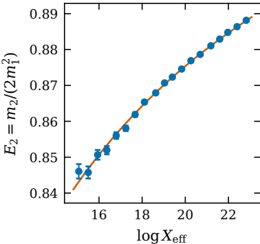
(a) \beta = 0.810
