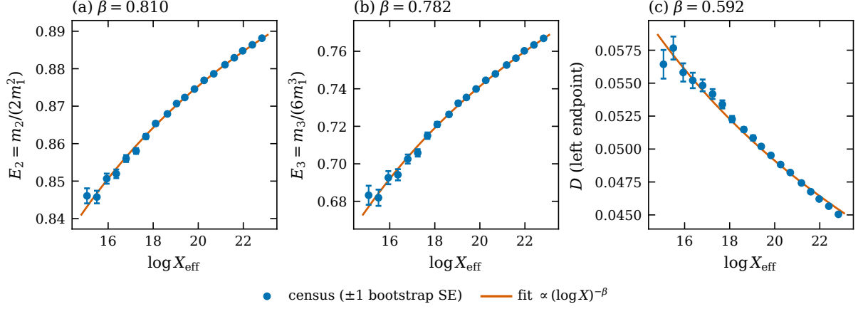
Figure 3: The local diagnostics against \log X_{\text{eff}} with bootstrap standard errors (mostly smaller than the markers) and the fitted power laws |\text{stat} - \text{limit}| \propto (\log X)^{-\beta} .
