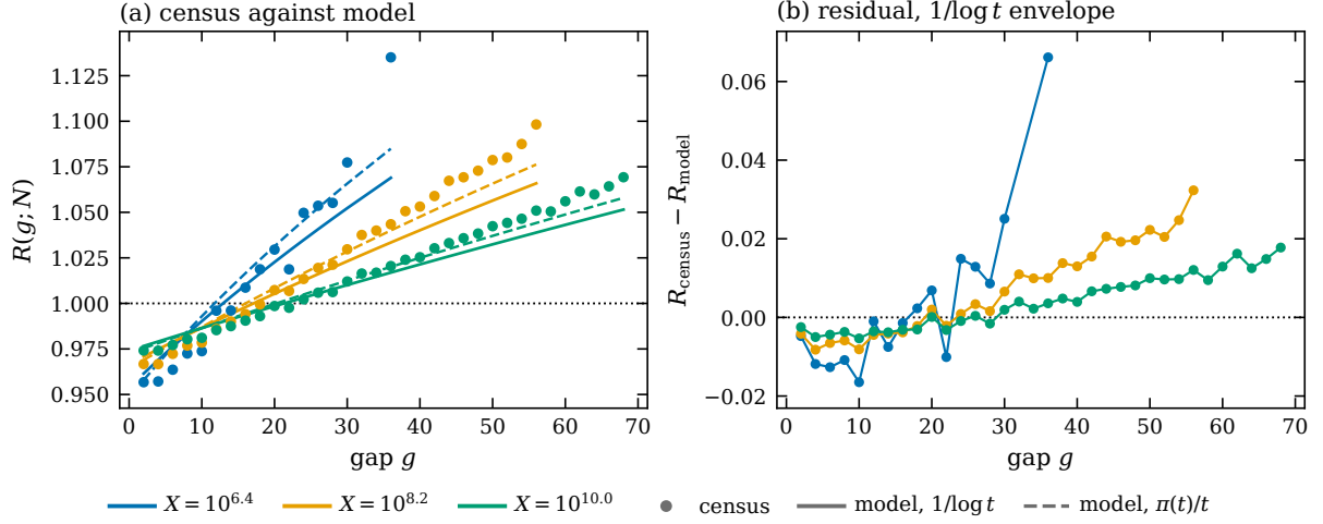
Figure 4: (a) R(g; N) at three scales against the parameter-free model with the 1/\log t envelope (solid) and the \pi(t)/t envelope (dashed). (b) Residual from the 1/\log t model; it shrinks with X in absolute terms because the whole effect scales as 1/\log X (see Figure 6(c) for the relative comparison).
