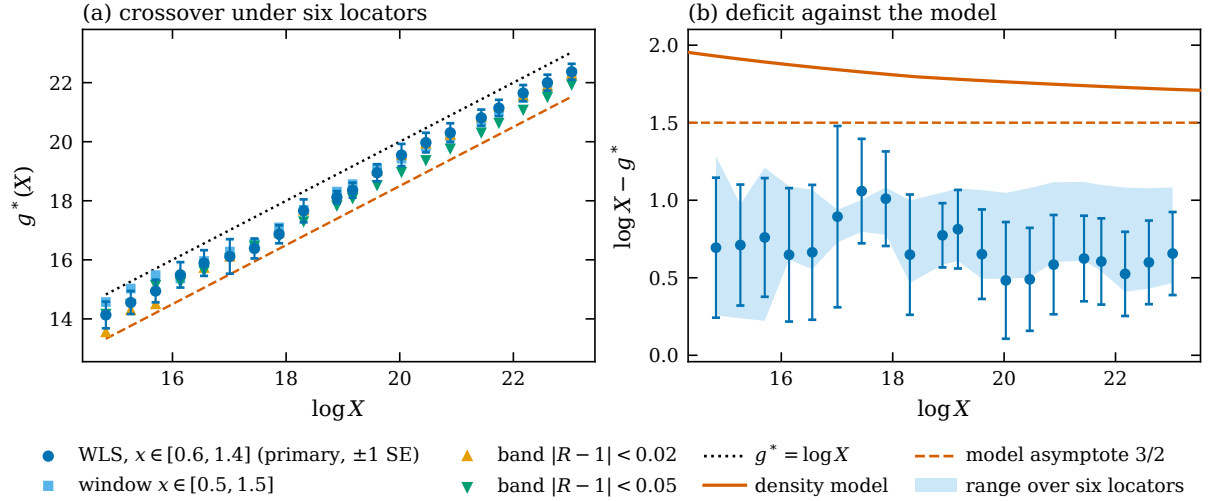
Figure 5: (a) The crossover g^*(X) under four of the six locators, with g^* = \log X and the model's asymptote g^* = \log X - 3/2 . (b) The deficit \log X - g^* : census (primary locator, with the range over all six locators shaded) against the numerical model. The model's O(1) constant is not reproduced.
