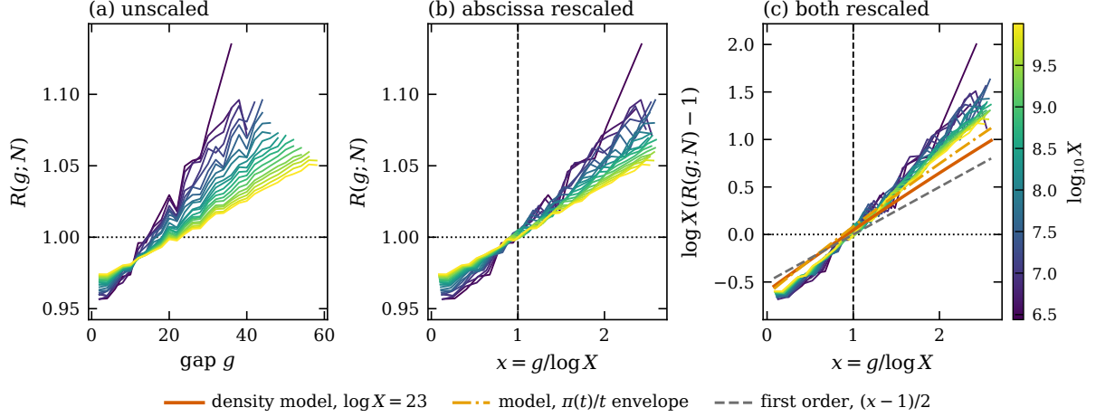
Figure 6: The scaling collapse. (a) R against g at all 20 scales; (b) abscissa rescaled by \log X ; (c) abscissa and amplitude rescaled. Panel (c) also shows the full numerical model at \log X = 23 for both envelopes and the first-order profile (x - 1)/2 : the model reproduces the crossing and the shape, not the slope.
