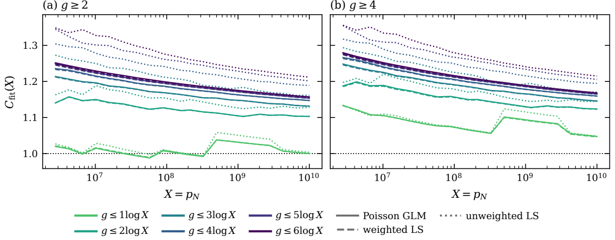
Figure 2: All 36 specifications across the 20 scales: colour is the window, line style the estimator. The vertical spread at fixed X exceeds the change of any one curve across the range.
