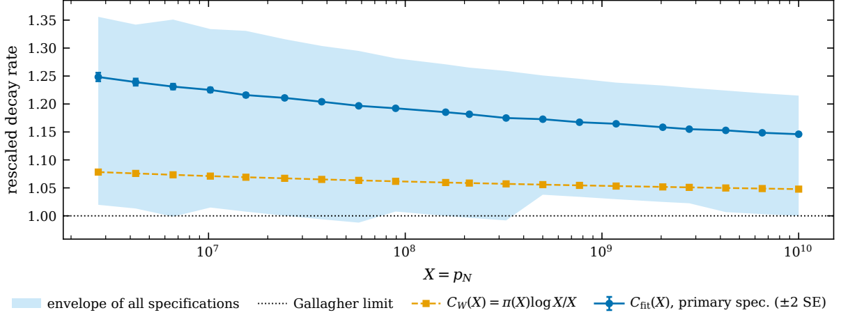
Figure 1: C_{\text{fit}}(X) under the primary specification, the envelope generated by all 36 specifications, and the benchmark C_W(X) . The envelope is wider at every scale than the change in any single specification across the whole range.
