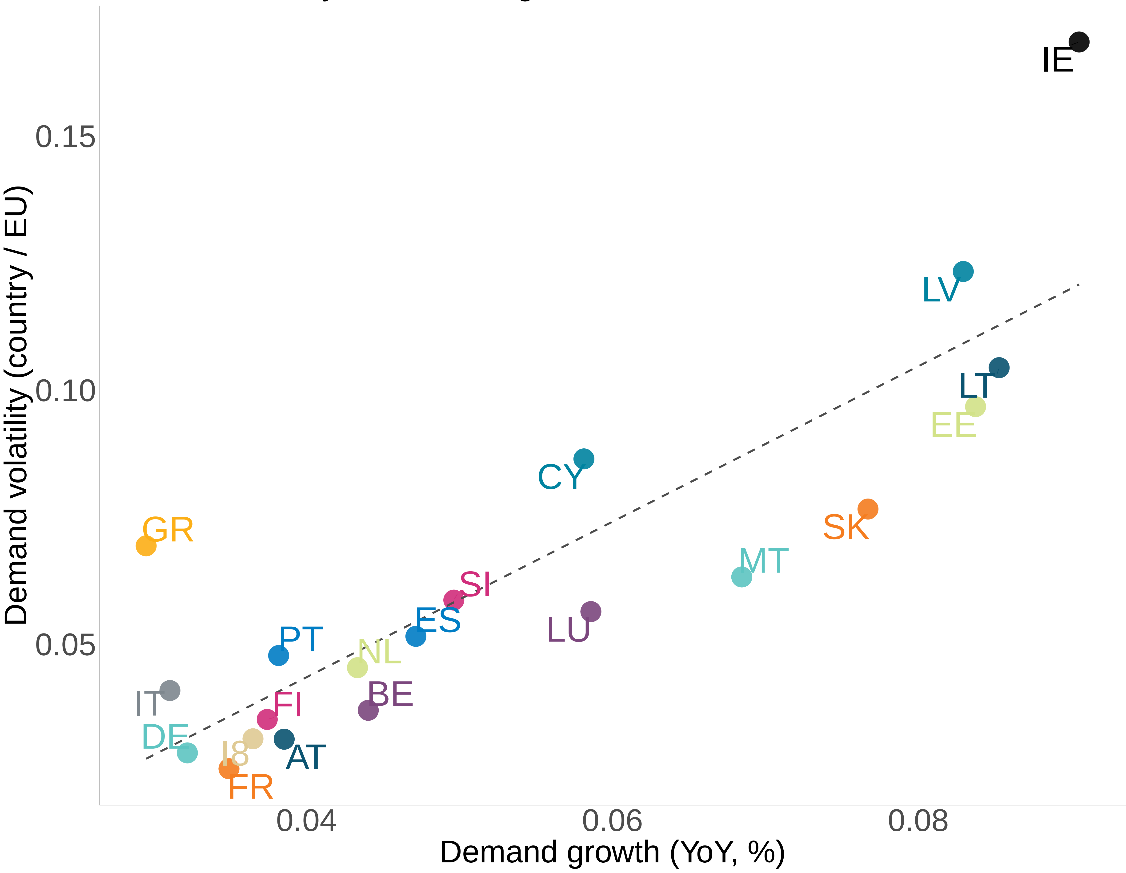
Demand volatility vs. demand growth
