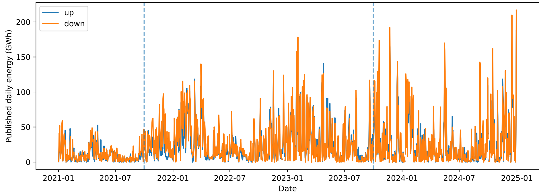
Reported upward and downward redispatch
