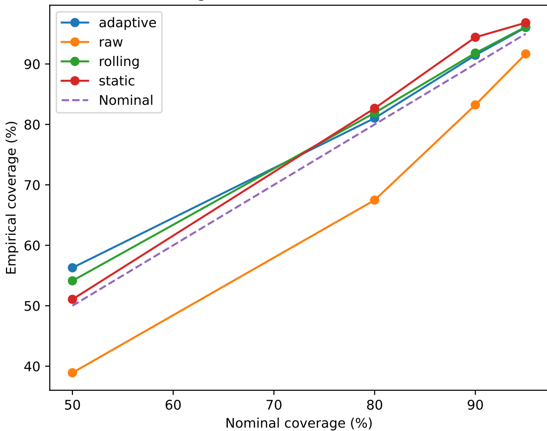
LightGBM interval calibration
