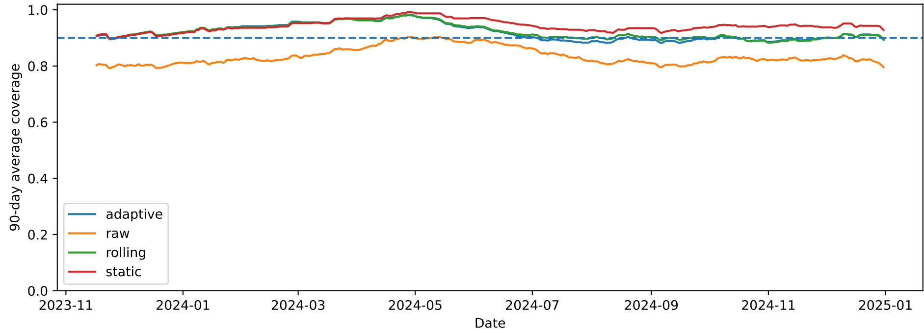
Coverage over time
