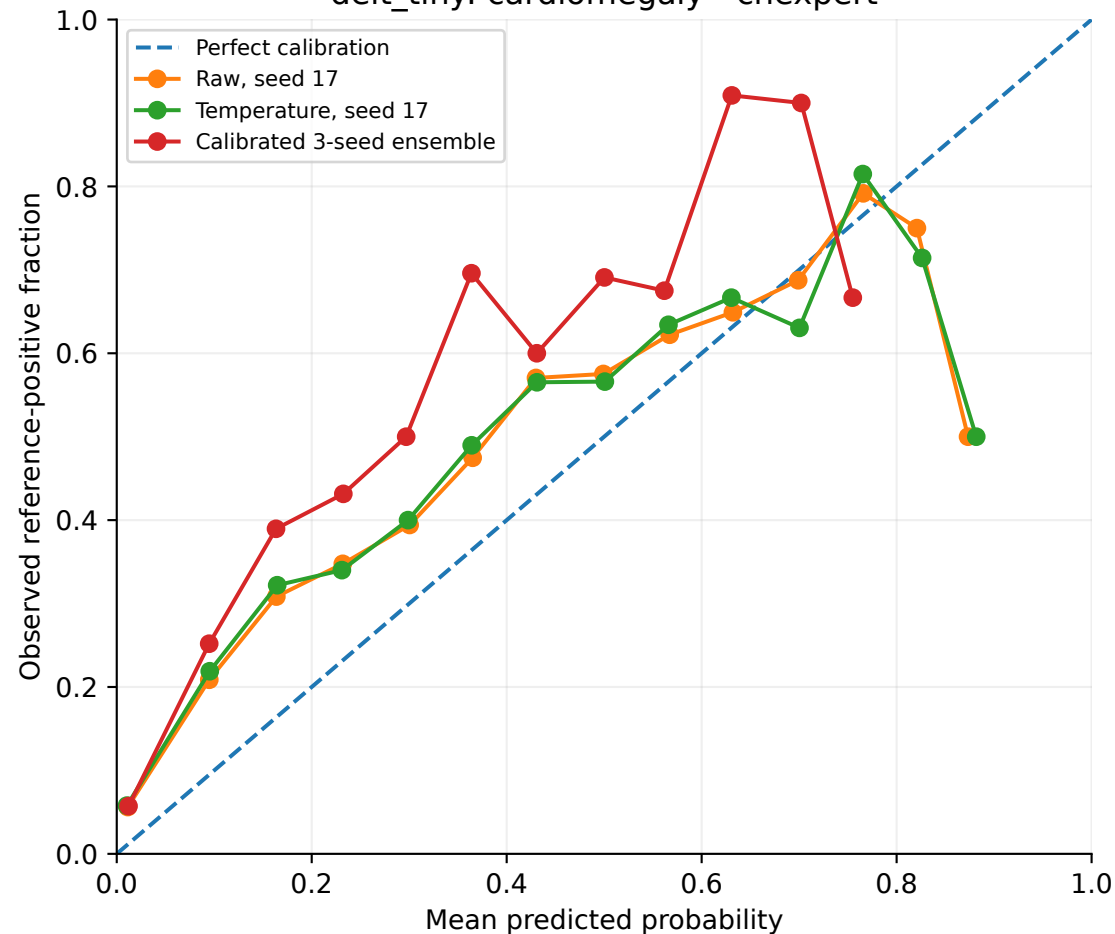
deit_tiny: cardiomegaly - chexpert
