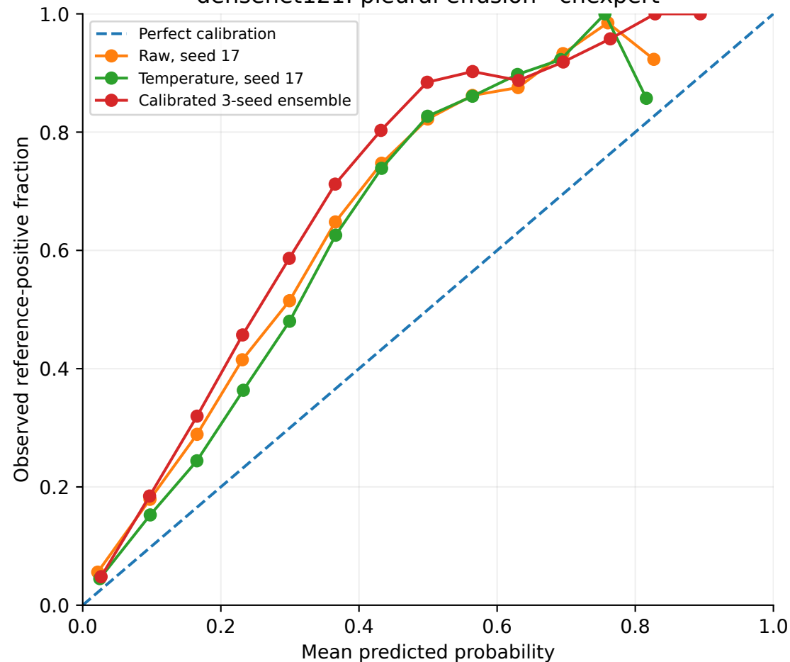
densenet121: pleural effusion - chexpert
