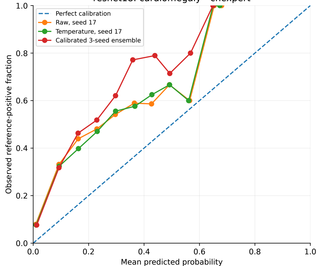
resnet18: cardiomegaly - chexpert
