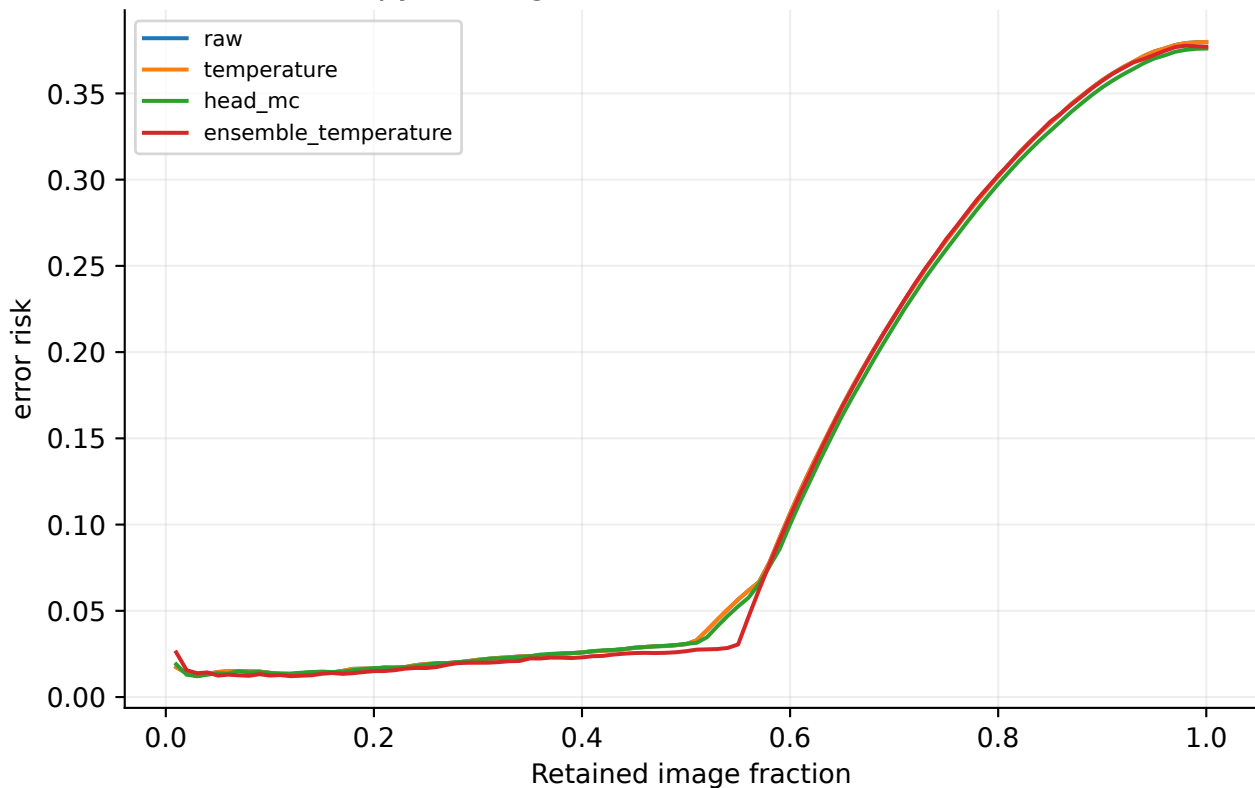
deit_tiny: cardiomegaly - chexpert Entropy ranking; source-frozen decision threshold
