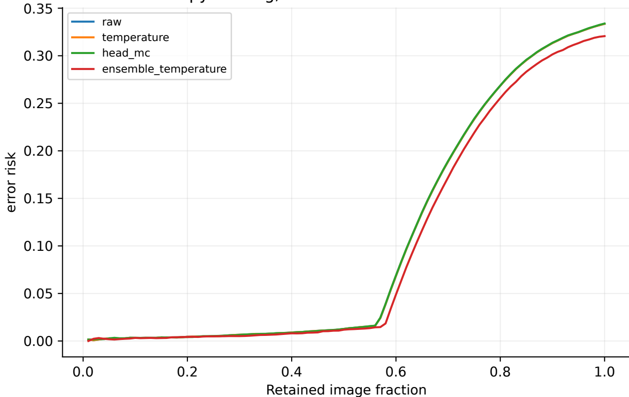
deit_tiny: pleural effusion - nih Entropy ranking; source-frozen decision threshold
