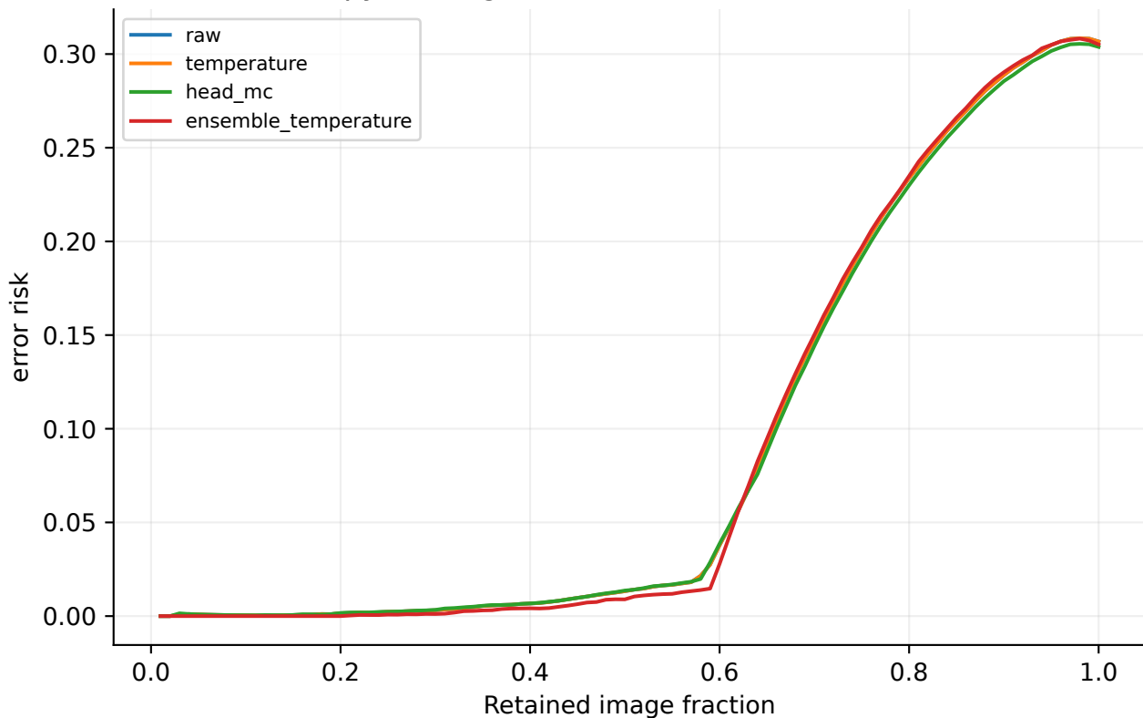
deit_tiny: cardiomegaly - vinbig Entropy ranking; source-frozen decision threshold
