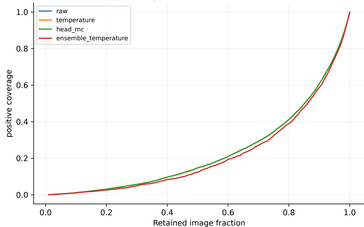
densenet121: cardiomegaly - chexpert Entropy ranking; source-frozen decision threshold
