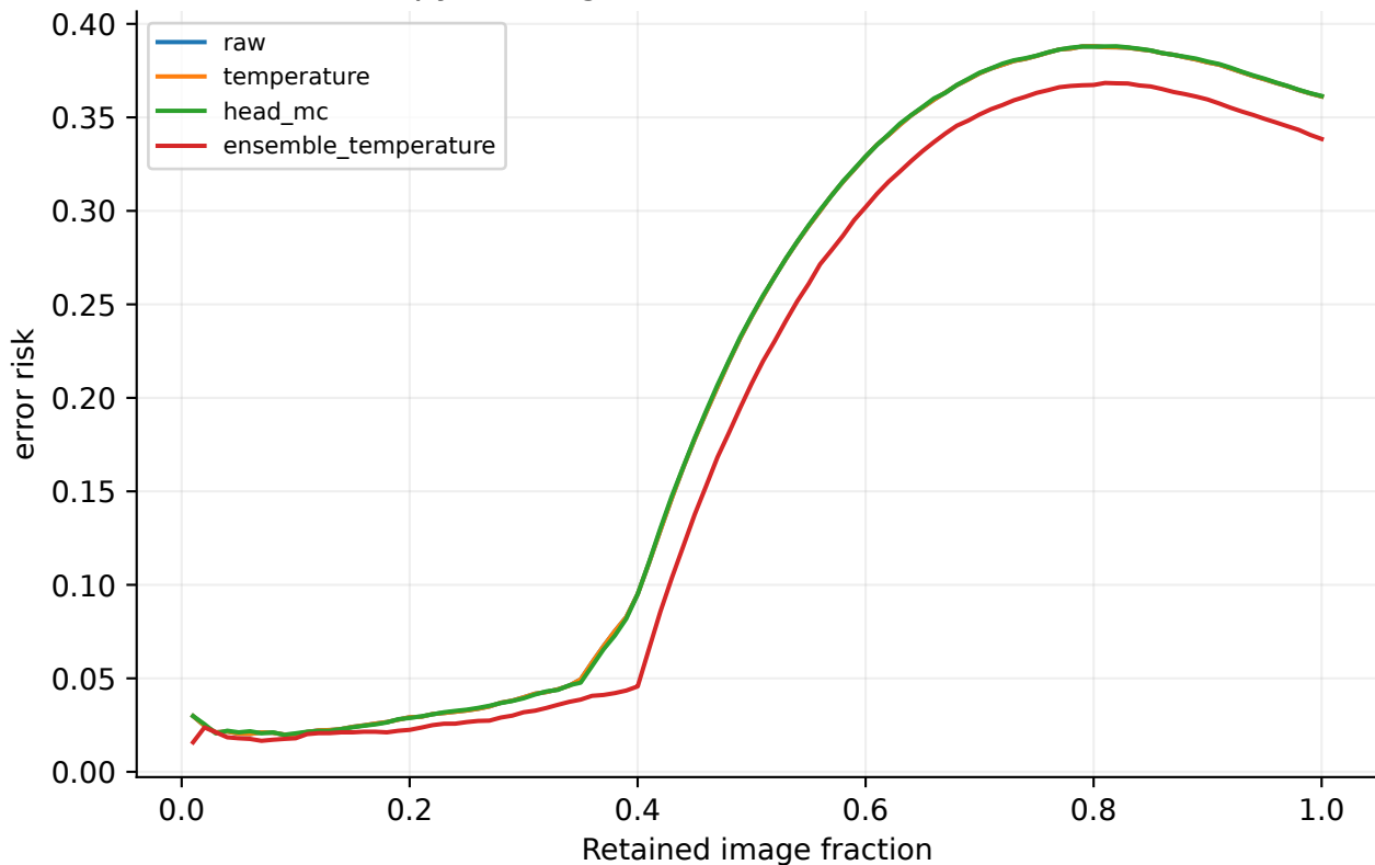
densenet121: pleural effusion - chexpert Entropy ranking; source-frozen decision threshold
