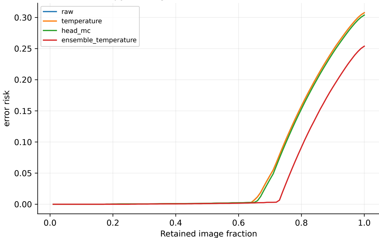
densenet121: cardiomegaly - nih Entropy ranking; source-frozen decision threshold
