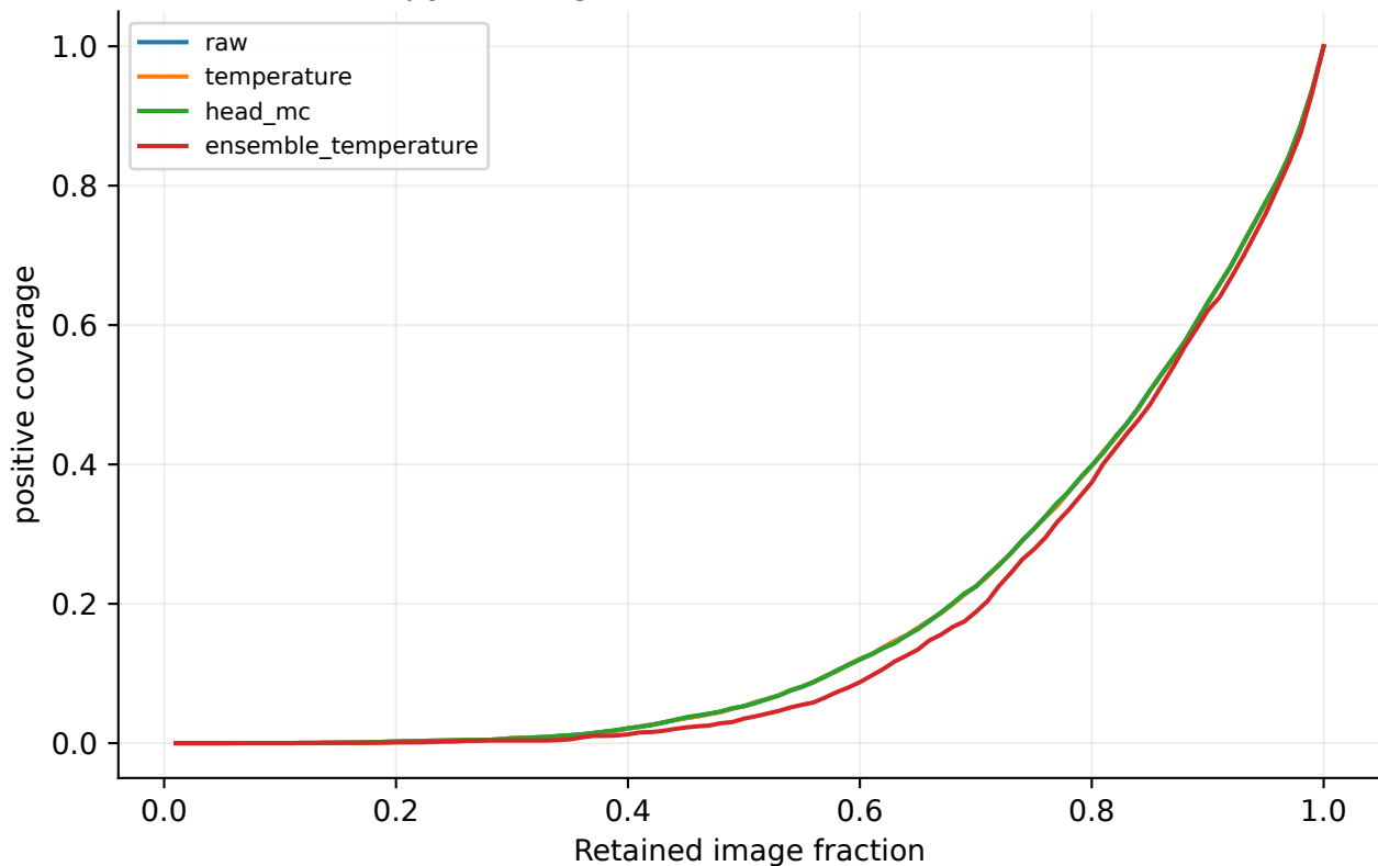
densenet121: cardiomegaly - vinbig Entropy ranking; source-frozen decision threshold
